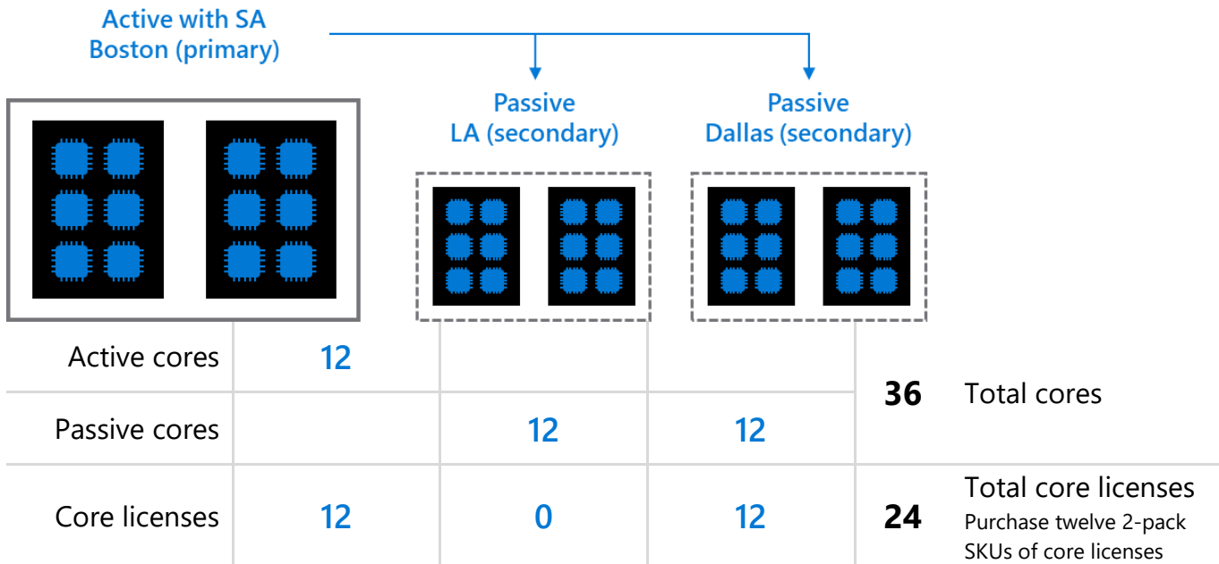
This figure shows an example of licensing an active primary SQL Server 2019 database with Software Assurance and multiple passive secondary databases.
