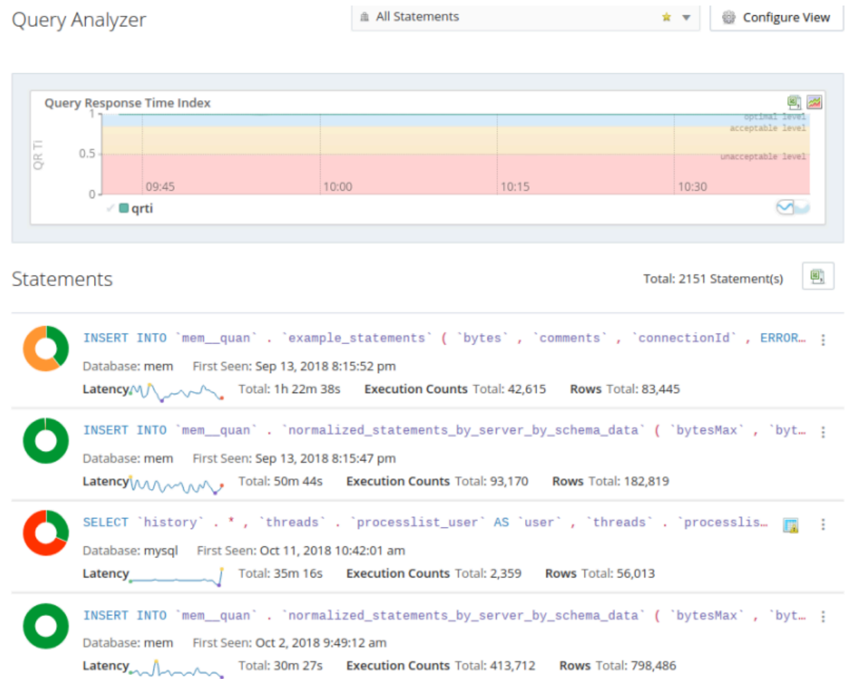
Figure 32.1 Default Query Analyzer View
