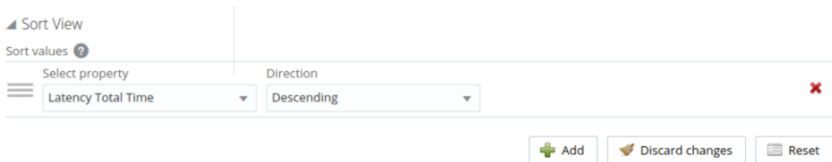
Figure 32.10 Sort View
