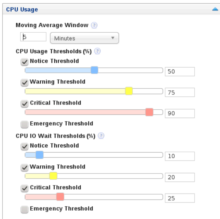
Figure 21.4 CPU Usage
