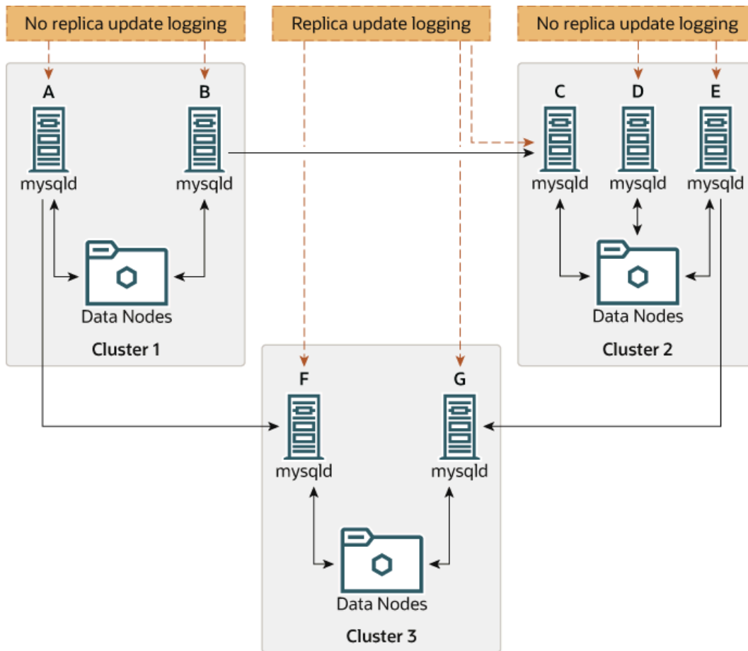
Figure 25.18 NDB Cluster Multi-Source Replication, With MySQL Servers
