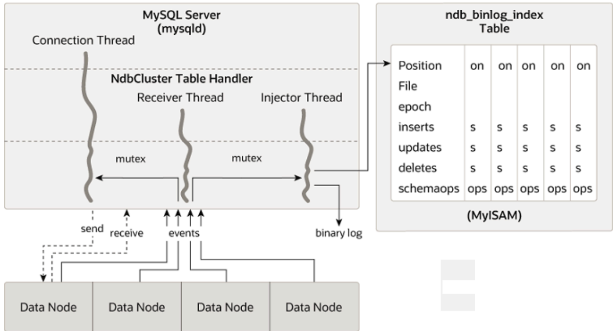
Figure 25.14 The Replication Source Cluster
