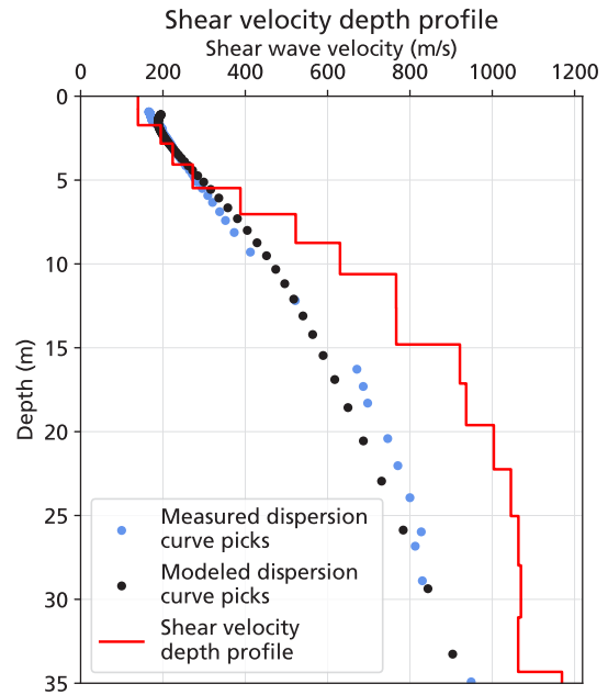
Above: Final Shear Velocity Depth Profiles (SVDP). If the final SVDP is based on the initial model, then only the measured dispersion curve picks are shown (blue dots).
