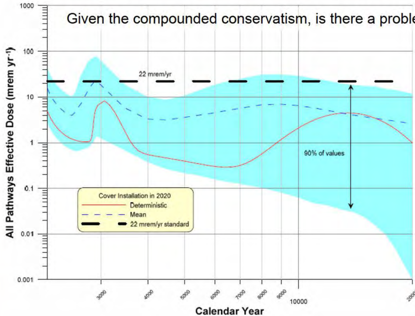
Figure 18 (Rood 2012)
