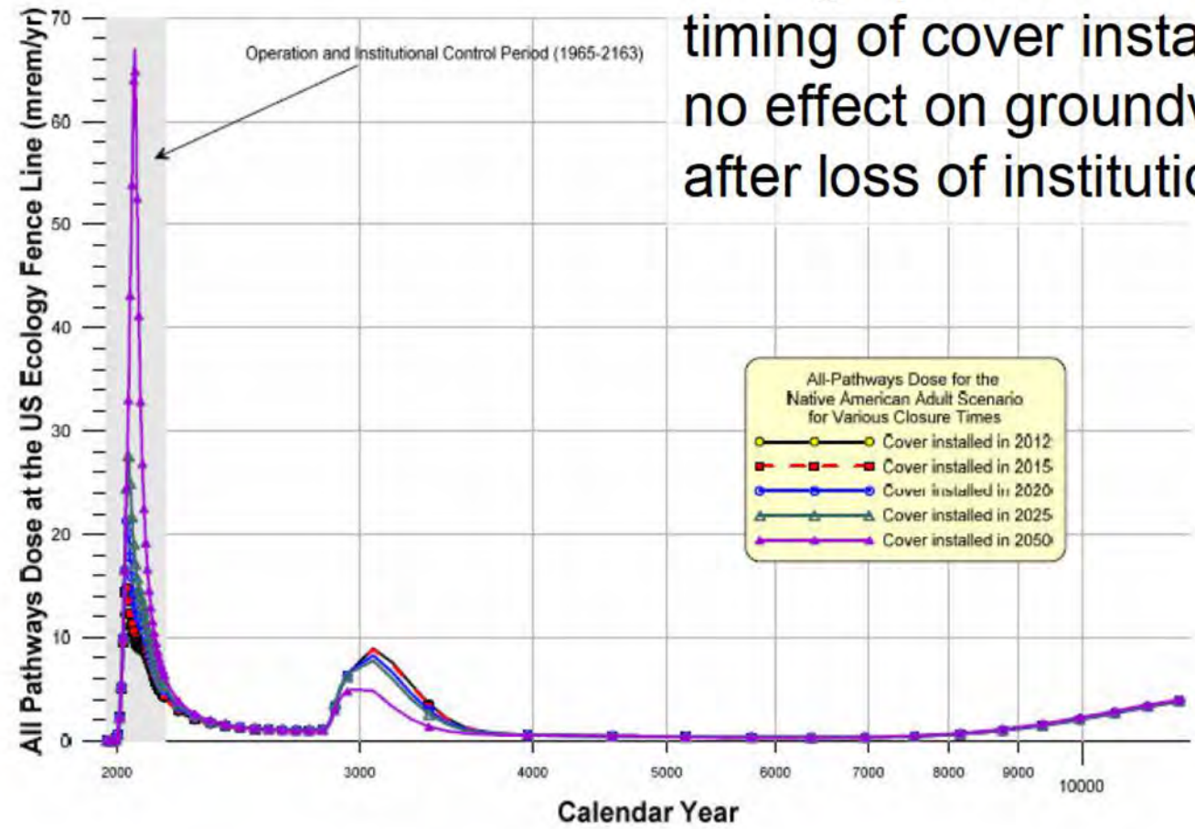
Figure 13 (Rood 2012)
