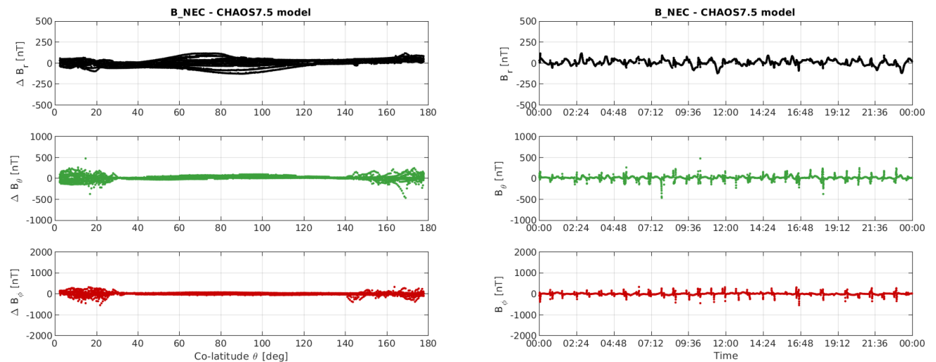
Figure 3-11: S/C B day 03.06: time series of B_{NEC} - B_{Chaos} residuals (right) and B_{NEC} - B_{Chaos} vs colatitude (left).
