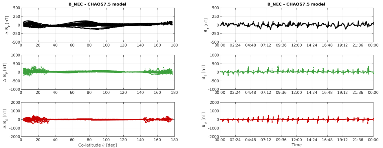
Figure 3-12: S/C C day 03.06: time series of B_{NEC} - B_{Chaos} residuals (right) and B_{NEC} - B_{Chaos} vs colatitude (left)
