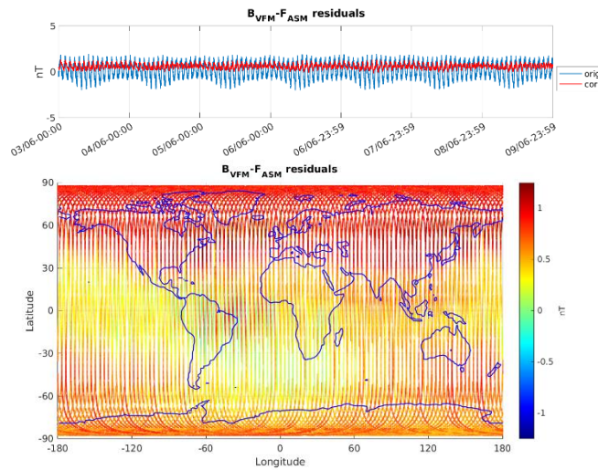
Figure 3-6: ASM-VFM residuals for S/C B, during monitoring period 03/06-09/06. In top figure are plotted: difference between |B_{VFM}| and F_{ASM} (without dB_{Sun} correction) (blue colour), and the residuals with dB_{Sun} corrections (red colour). In bottom figure residuals are presented on the world map.
