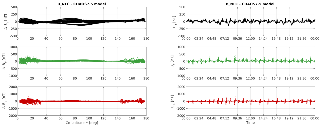
Figure 3-10: S/C A day 03.06: time series of B_{NEC} - B_{Chaos} residuals (right) and B_{NEC} - B_{Chaos} vs colatitude (left).
