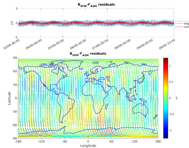
Figure 3-5: ASM-VFM residuals for S/C A, during monitoring period 03/06-09/06. In top figure are plotted: difference between |B_{VFM}| and F_{ASM} (without dB_{Sun} correction) (blue colour), and the residuals with dB_{Sun} corrections (red colour). In bottom figure residuals are presented on the world map.
