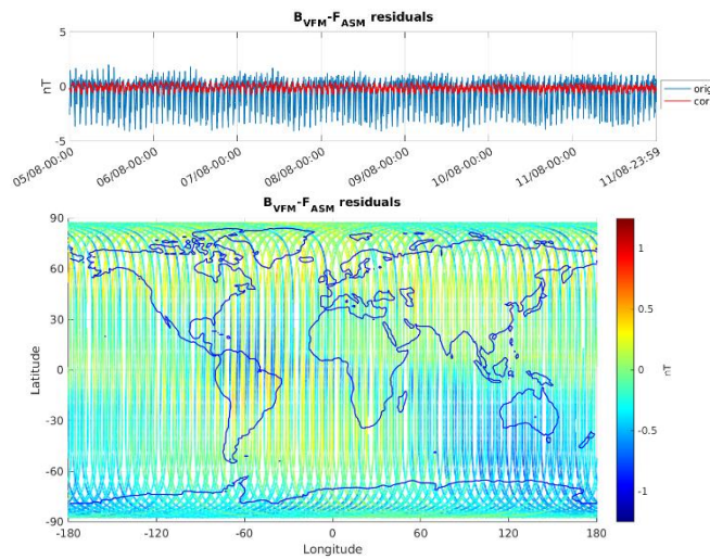
Figure 3-5: ASM-VFM residuals for S/C A, during monitoring period 05/08-11/08. In top figure are plotted: difference between |B_{VFM}| and F_{ASM} (without dB_{Sun} correction) (blue colour), and the residuals with dB_{Sun} corrections (red colour). In bottom figure residuals are presented on the world map.
