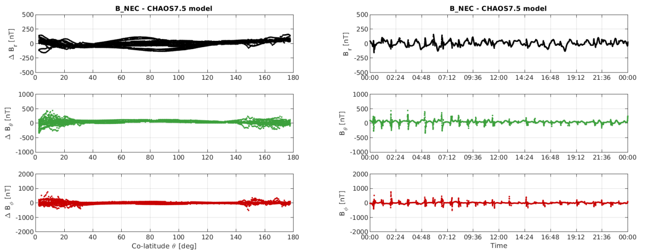
Figure 3-11: S/C B day 05/08: time series of B_{NEC} - B_{Chaos} residuals (right) and B_{NEC} - B_{Chaos} vs colatitude (left).
