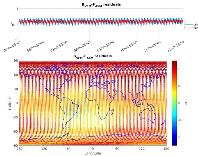
Figure 3-6: ASM-VFM residuals for S/C B, during monitoring period 05/08-11/08. In top figure are plotted: difference between |B_{VFM}| and F_{ASM} (without dB_{Sun} correction) (blue colour), and the residuals with dB_{Sun} corrections (red colour). In bottom figure residuals are presented on the world map.
