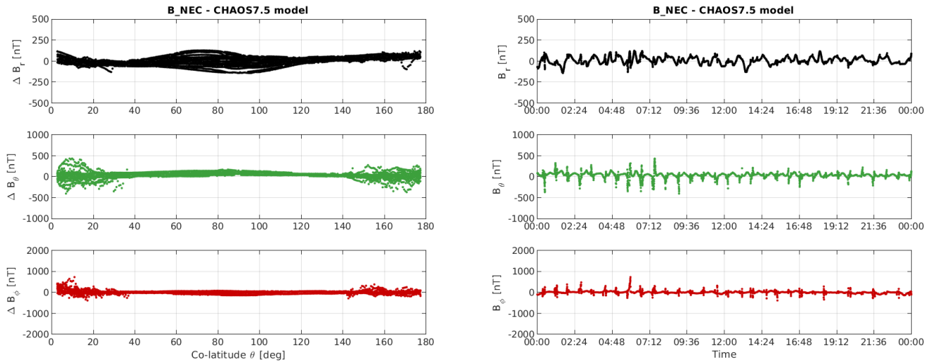
Figure 3-12: S/C C day 05/08: time series of B_{NEC} - B_{Chaos} residuals (right) and B_{NEC} - B_{Chaos} vs colatitude (left)
