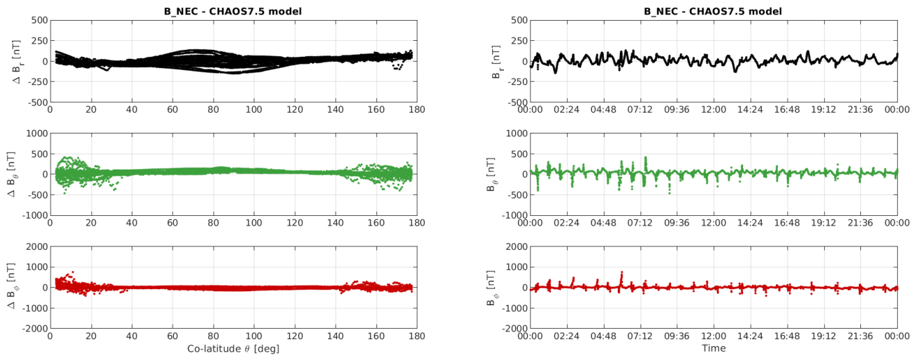
Figure 3-10: S/C A day 05/08: time series of B_{NEC} - B_{Chaos} residuals (right) and B_{NEC} - B_{Chaos} vs colatitude (left).
