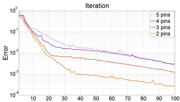
Figure 12: Example convergence plot of an IK solve with different pin numbers. All soft and hard constraints are included in this example.
