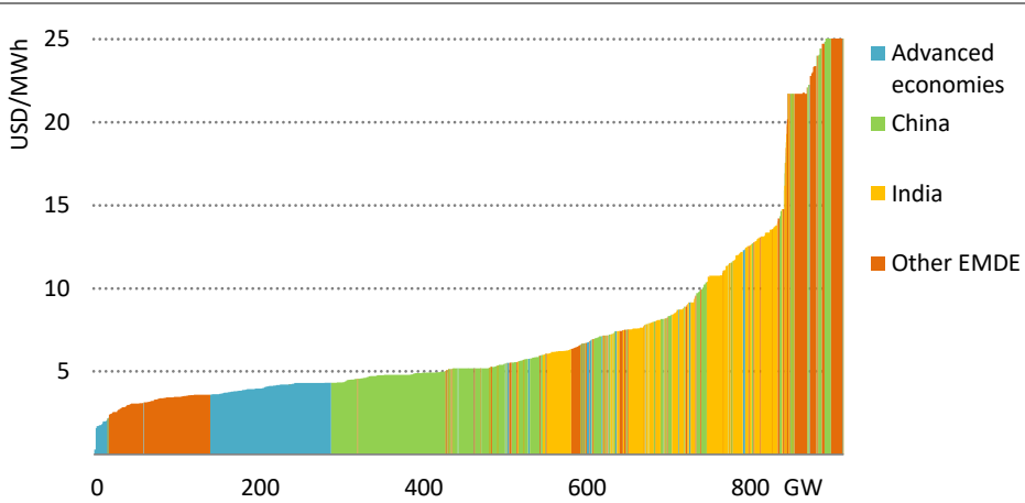
Figure 4.19 ▶ Increase in capital recovery costs to align the coal fleet with lower plant utilisation rates in the APS
