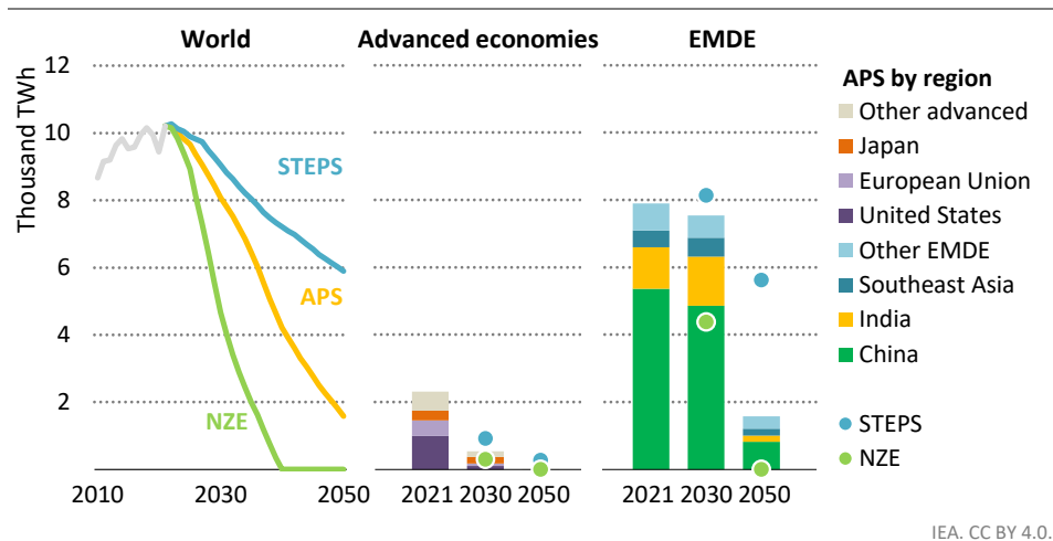
Figure 2.1 ▶ Unabated coal-fired electricity generation by region and scenario, 2010-2050
