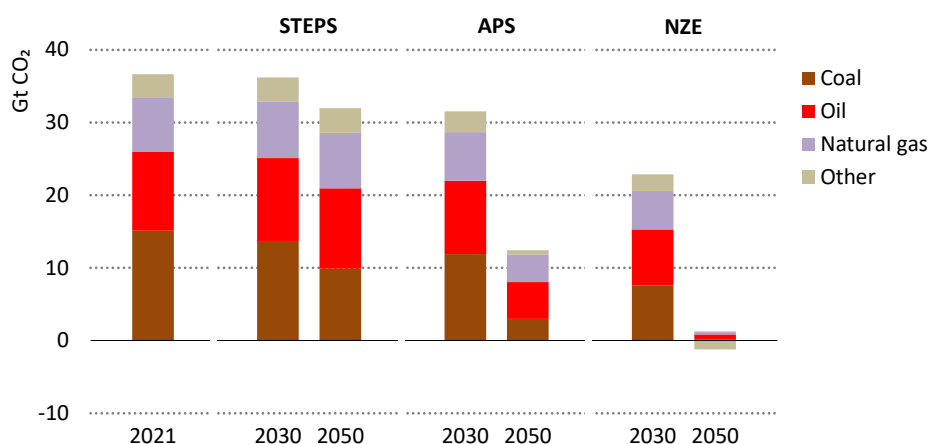
Figure 1.18 ▶ CO 2 emissions by source and scenario
