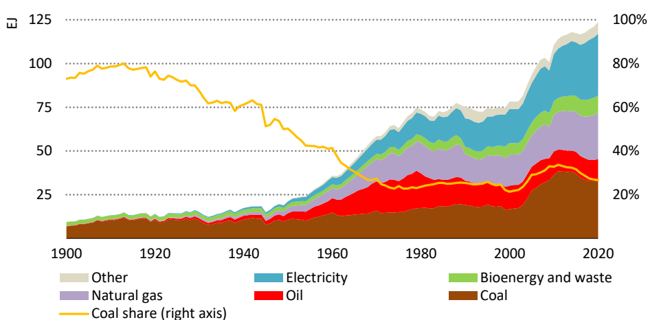
Figure 3.3 ▶ Final energy consumption in industry, 1900-2020
