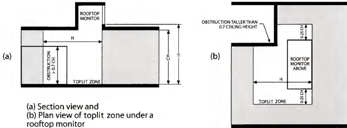
FIGURE C405.2.4.3(2)
