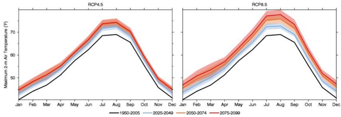
Figure 7: Projected changes to maximum temperatures in Jefferson County 52 .
