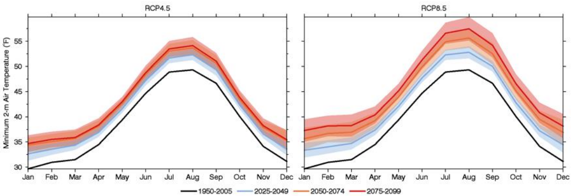
Figure 9: Projected changes to minimum temperatures in Jefferson County 54 .
