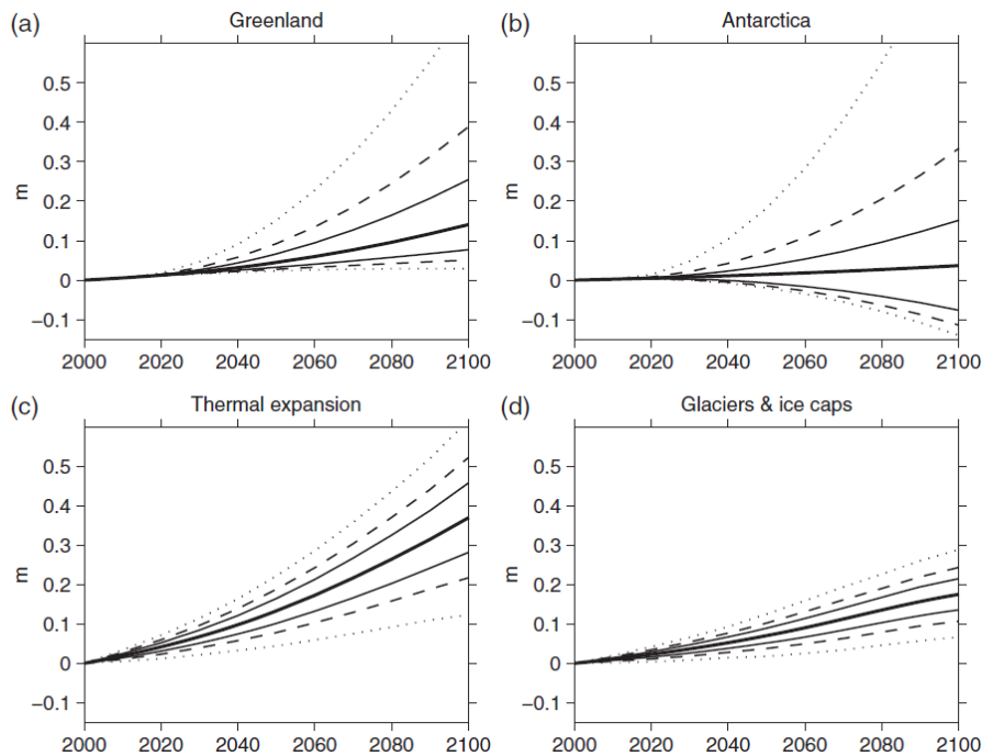
Figure 15: Projections of cumulative contribution of (a) the Greenland ice sheet, (b) the Antarctic ice sheet, (c) thermal expansion, and (d) glaciers to global sea-level rise under RCP 8.5 81 . Heavy line=median, light line = 67% range, dashed = 5th-95th percentile; dotted = 0.5 th -99.5 th percentiles. Y-axis units are in Meters (M), and 0.1M = approximately 4 inches.
