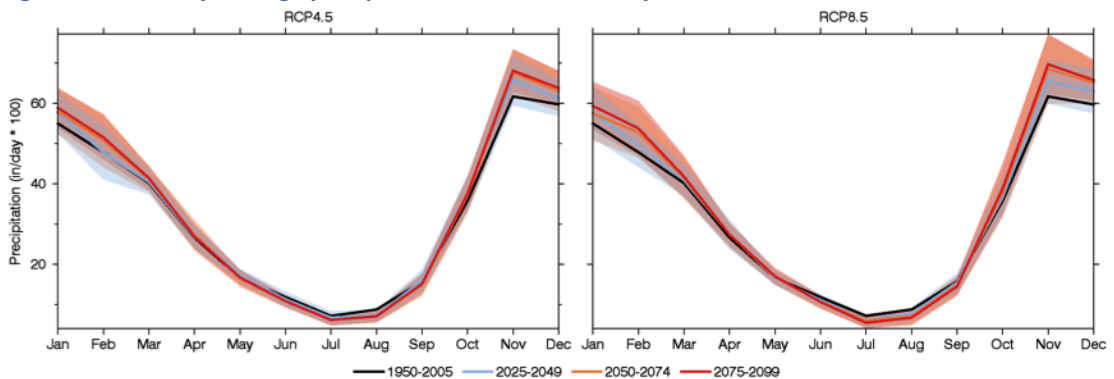
Figure 12: Monthly average precipitation in Jefferson County 67 .
