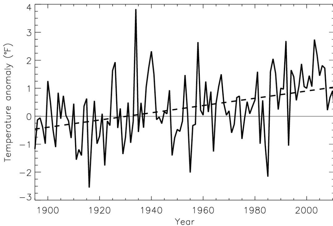
Figure 4: Average annual temperature anomaly (changes from the 1901-1960 average) in the Pacific Northwest 47 .
