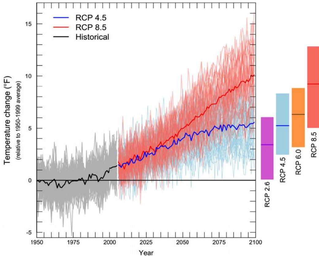
Figure 5: Observed and projected changes in temperature for the Pacific Northwest. Observed (1950-2011) regional mean annual temperature increases are shown in gray, and projected increases in blue and red (blue for a lower greenhouse gas emission scenario - RCP 4.5, and red for a higher greenhouse gas emissions scenario – RCP 8.5). Average annual temperature for the 2050s is projected to increase 4.5°F (RCP 4.5 - range 2.0°F to 6.7°F) to 5.8°F (RCP 8.5 -range 3.1°F to 8.5°F) relative to 1950-1999 50
