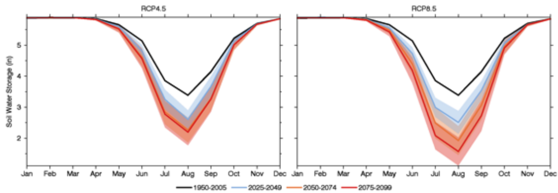
Figure 31: Projected changes to soil water storage in Jefferson County 106 . Monthly averages of soil water storage for four time periods for the RCP4.5 and RCP 8.5 future emission scenario.
