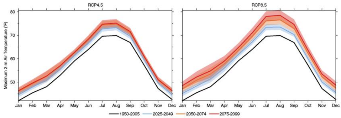
Figure 6: Projected changes to maximum temperatures in Clallam County 51 .
