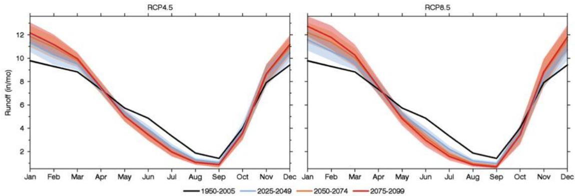
Figure 13: Monthly average runoff in Clallam County 69 .
