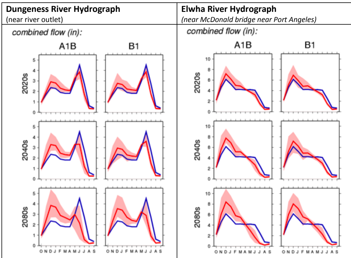
Figure 35: Hydrograph projections for the Dungeness and Elwha rivers 124 . The blue line is the historical flow, while the red line is the projected average flow with the red shading showing variability. Flow amount is shown with monthly values, starting in October and ending in September. The A1B scenario is similar to the RCP 8.5 scenario and represents the “business as usual” scenario where little attempt is made at greenhouse gas (GHGs) emissions reductions, the B1 scenario is similar to the RCP 4.5 scenario and represents a future where reductions in current amounts of GHGs are undertaken. A detailed illustration of the GHG assumptions between scenarios is available in Figure 3.
