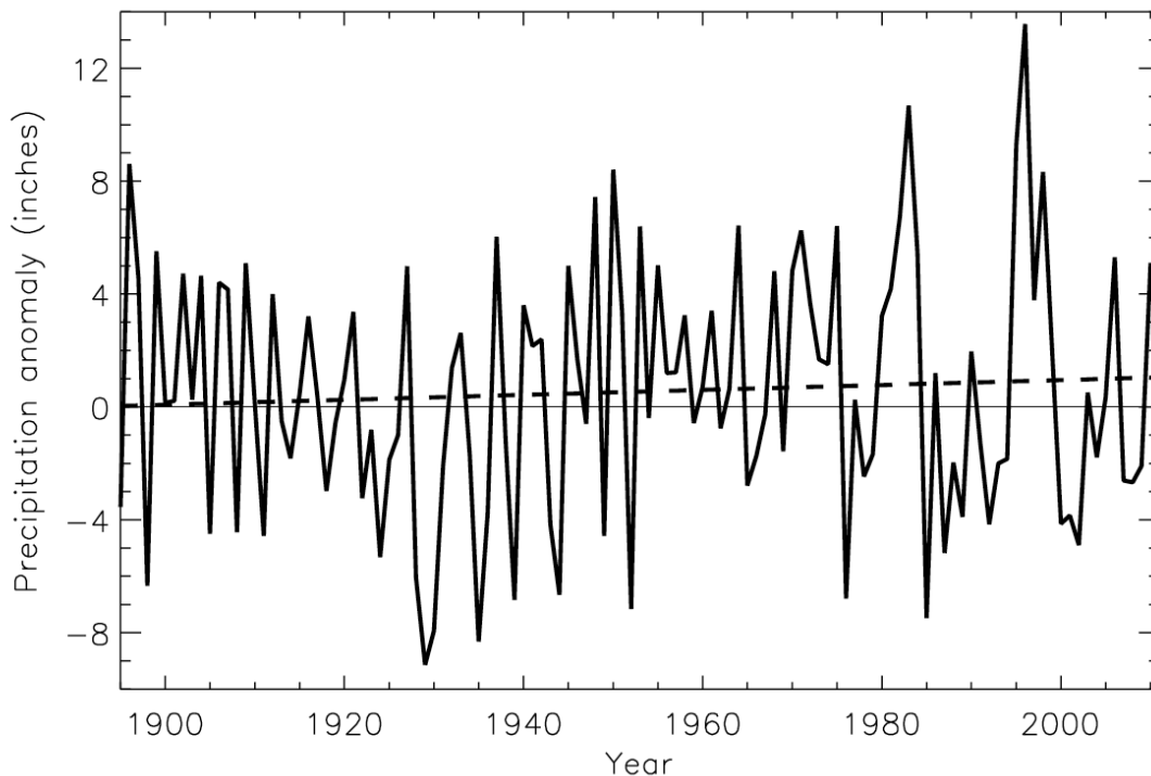
Figure 10: Average annual precipitation anomaly (changes from the 1901-1960 average) in the Pacific Northwest 60 . Trend line (dashed) is not statistically significant (i.e. not different than zero).
