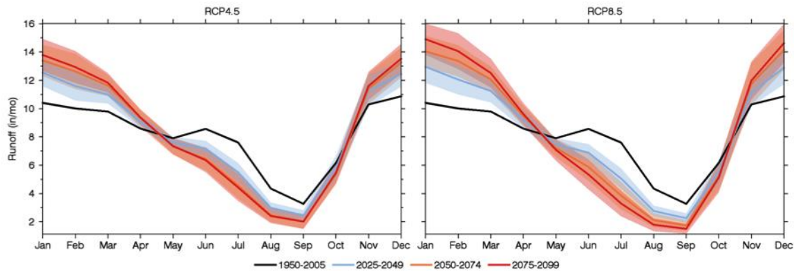
Figure 14: Monthly average runoff in Jefferson County 70 .
