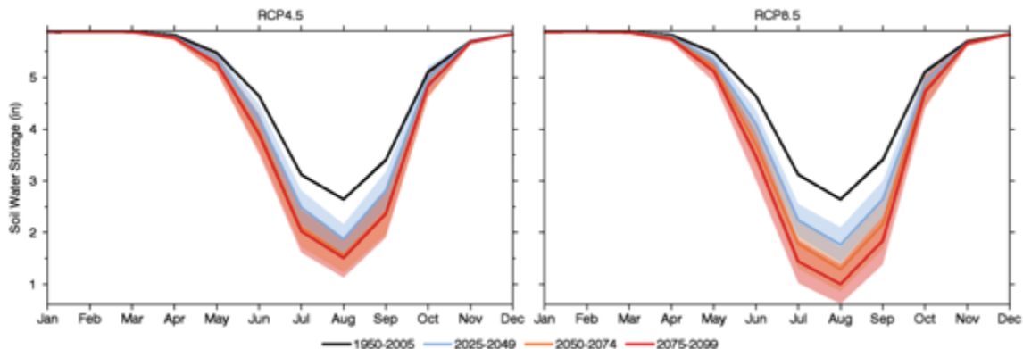
Figure 30: Projected changes to soil water storage in Clallam County 105 . Monthly averages of soil water storage for four time periods for the RCP4.5 and RCP 8.5 future emission scenarios.
