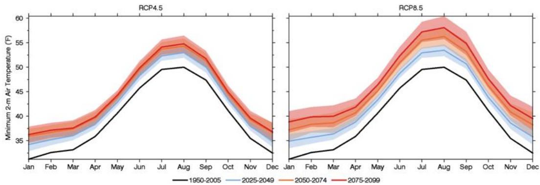
Figure 8: Projected changes to minimum temperatures in Clallam County 53 .
