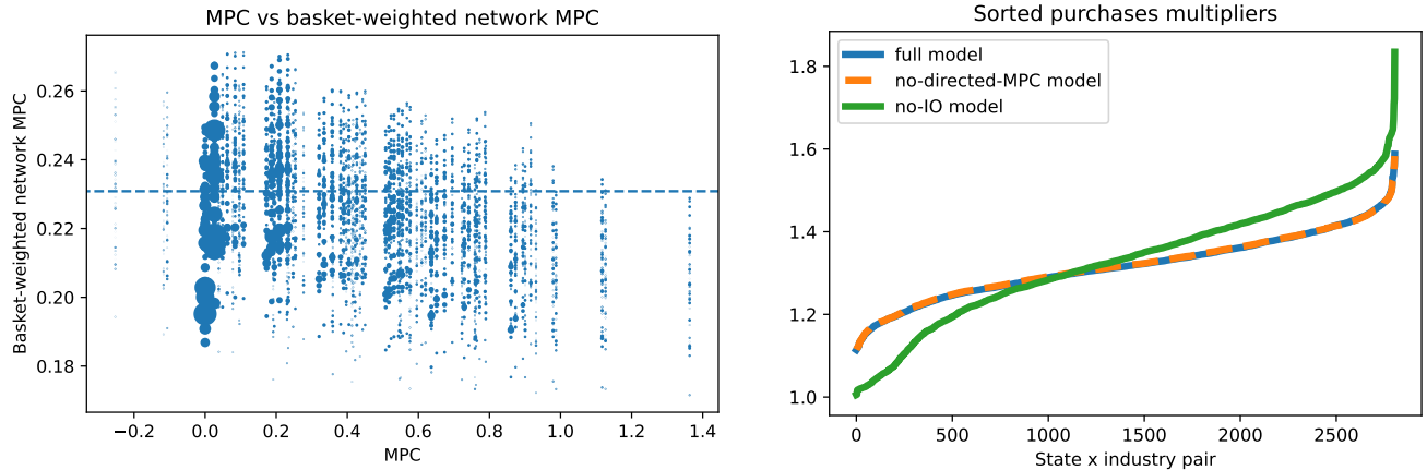
Fig. 3. The left panel shows a scatter of MPCs m_n against basket-weighted MPCs m_n^{next} . The dashed line gives the average MPC E_{h^*}[m_n] for h^* given by the income incidence of a shock to demand proportional to 2012 state-industry GDP. The right panel shows the change in aggregate consumption for each industry-region pair according to a one dollar demand shock in each pair, sorted by the magnitude of the effect. The full model is the baseline and plotted in blue. The no-directed-MPC model assumes that all households direct their consumption in proportion to aggregate consumption. The no-IO assumes that there is no use of intermediate goods.
