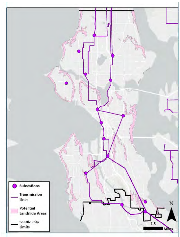
Figure 23. Landside Risk to Transmission Lines and Substations
