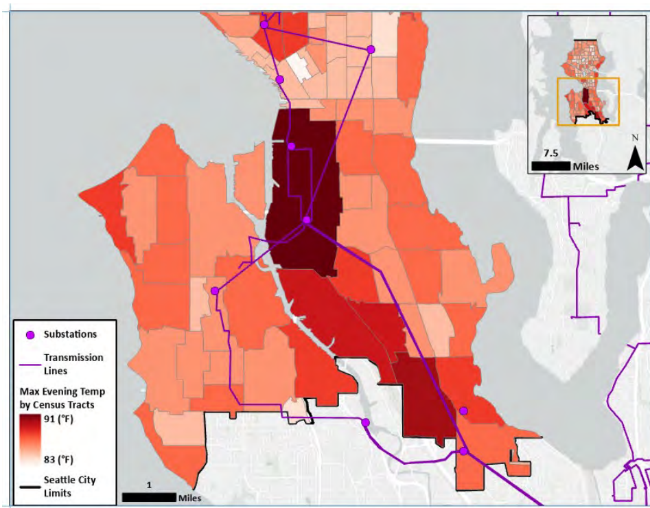
Figure 24. Extreme Heat and Energy Infrastructure in Seattle
