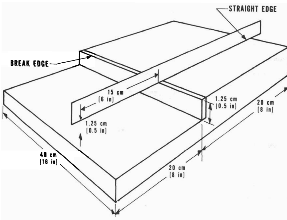
FIGURE 1. Break fixture.
