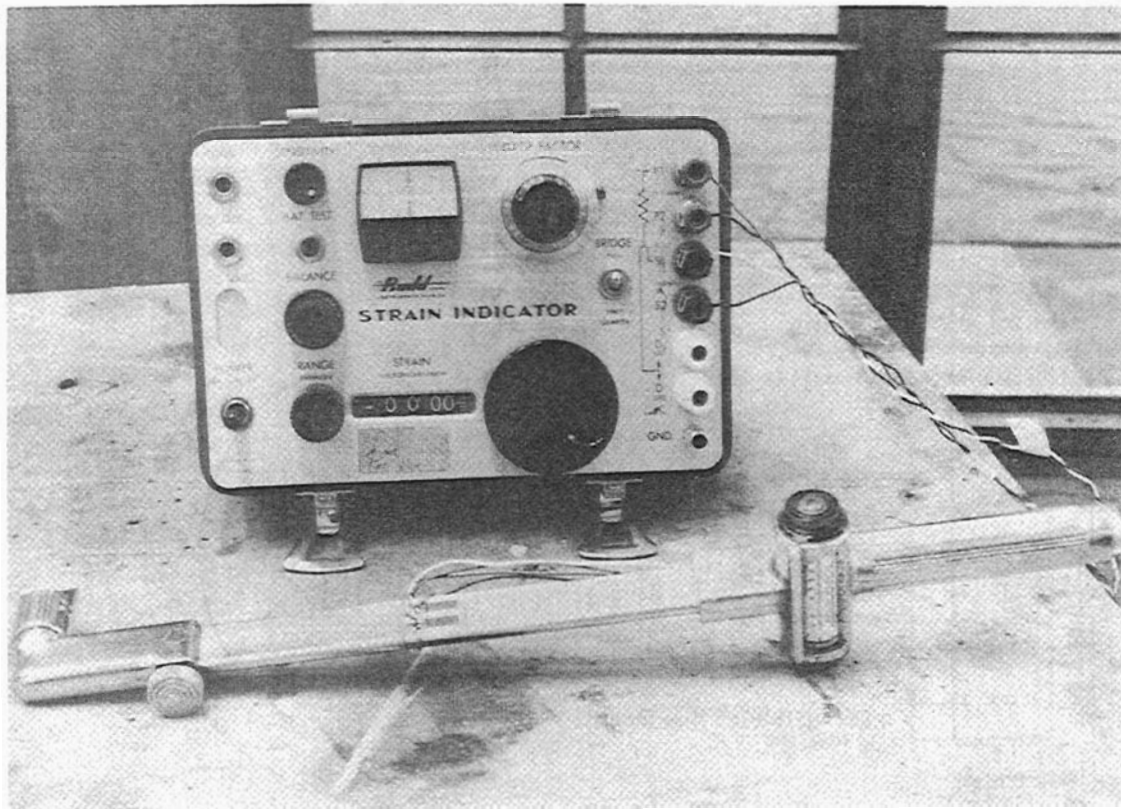
Figure B-8. Torque Applicator System.
