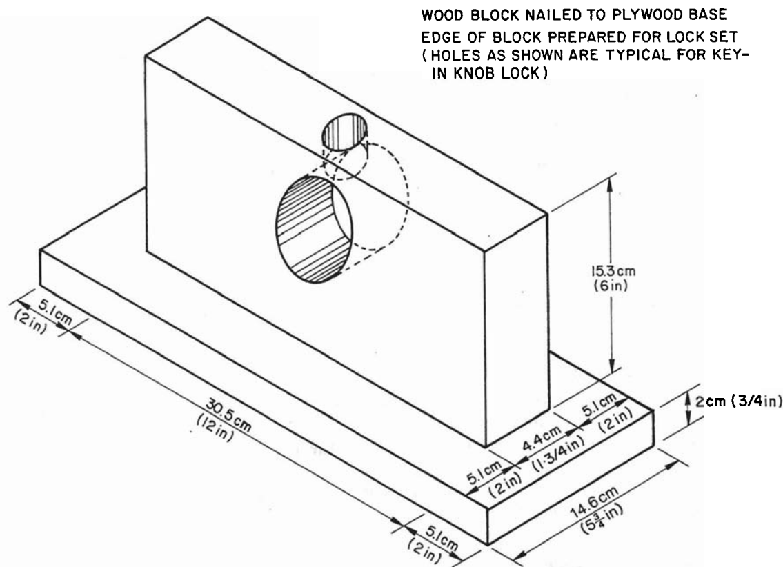
Figure 4. Bolt Pressure Test Fixture
