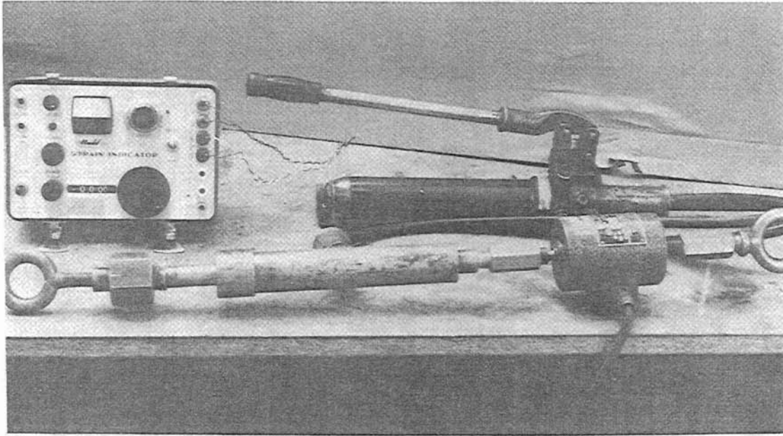
Figure B-11. Hydraulic Ram and Load Cell.
