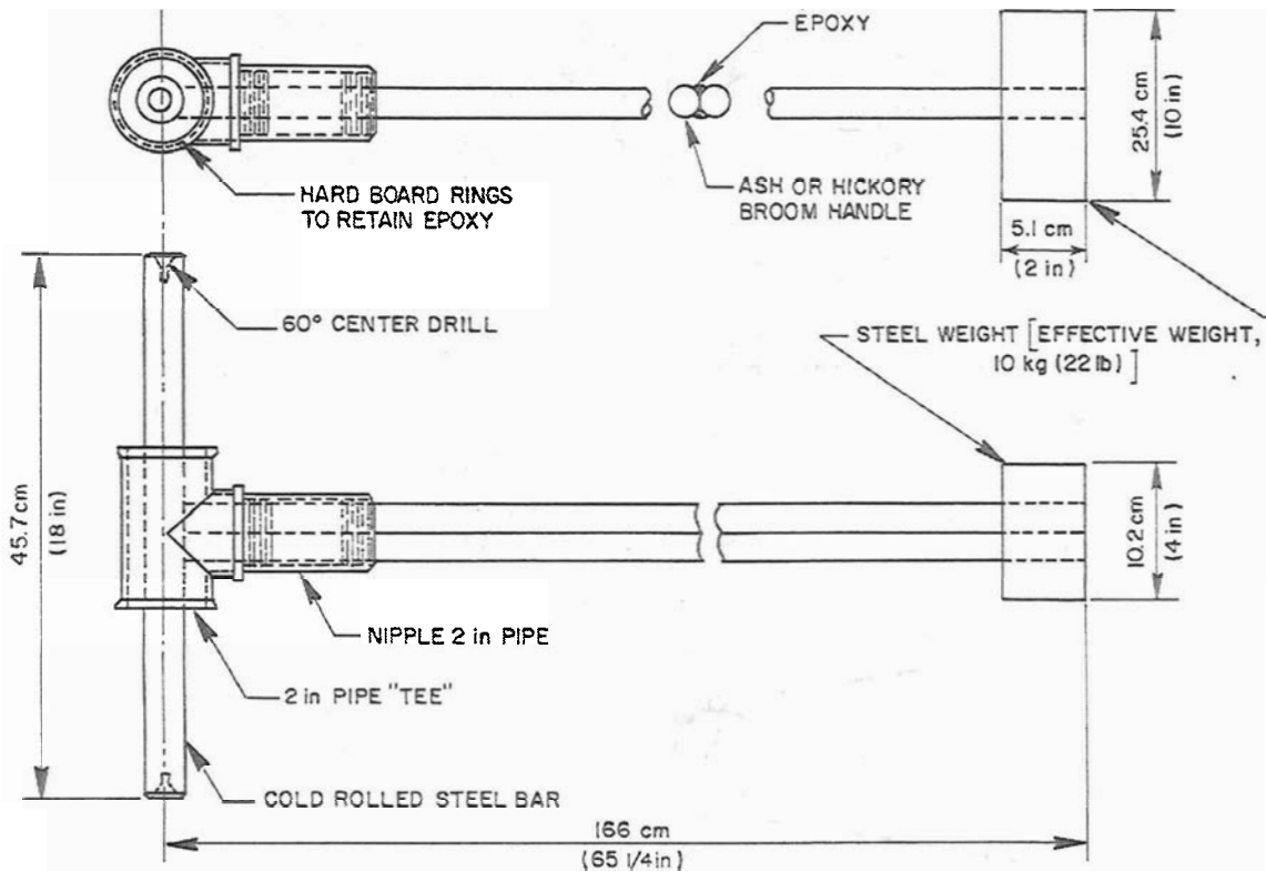
Figure B-6. Vertical Impactor
