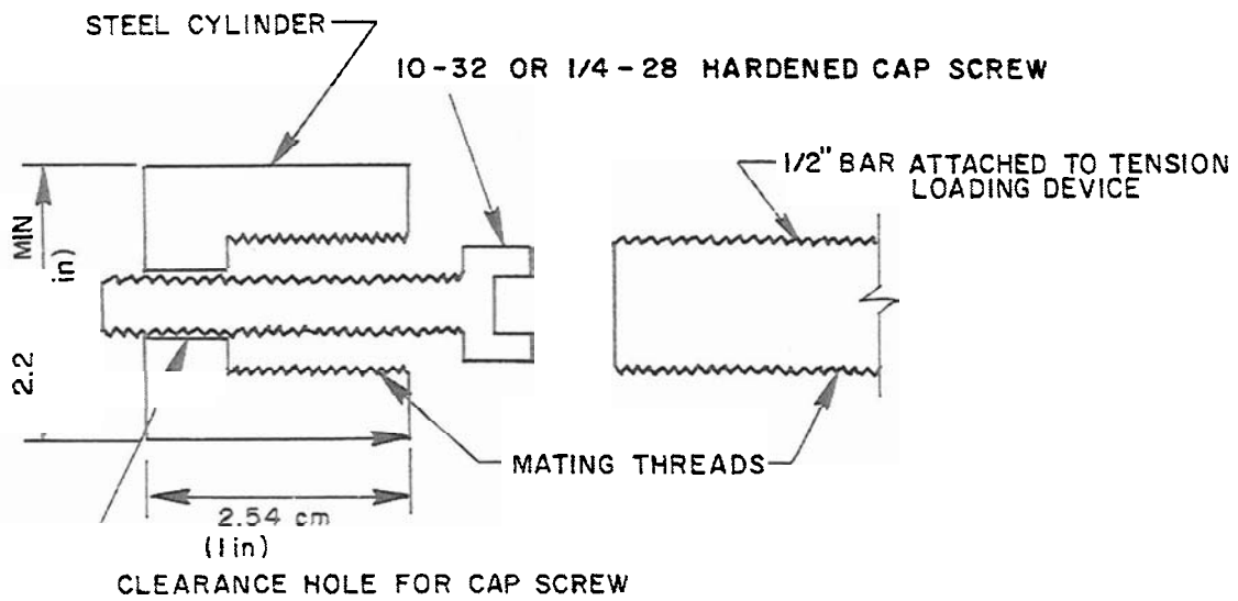
Figure B-12. Tension Loading Adapter
