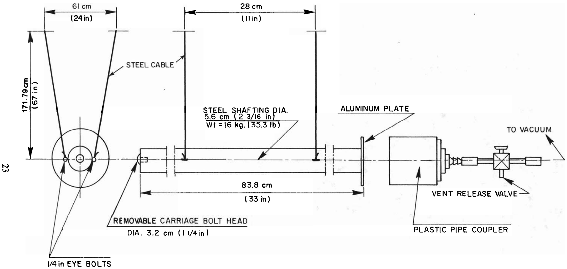
Figure B-4. Component Ram.
