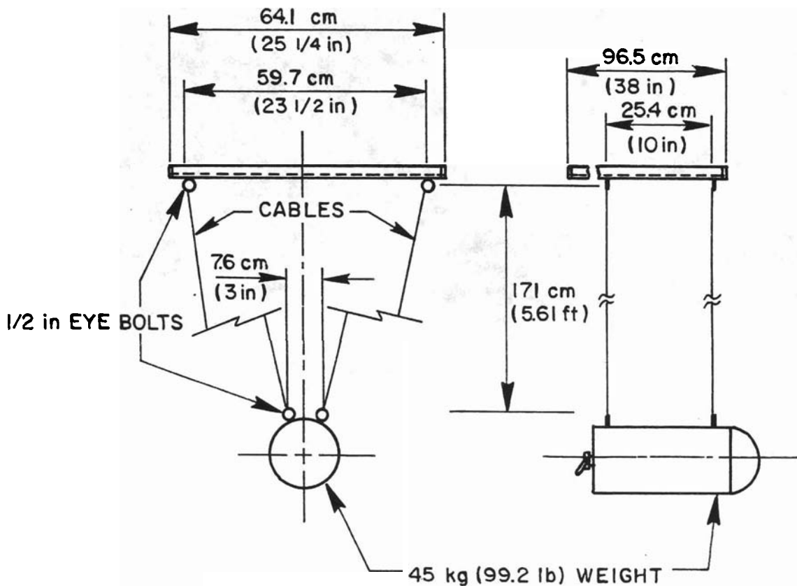
Figure B-3. Door Ram Suspension System
