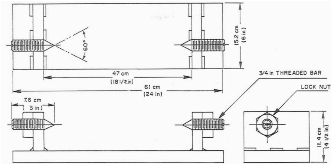
Figure B-7. Vertical Impactor Pivot Assembly
