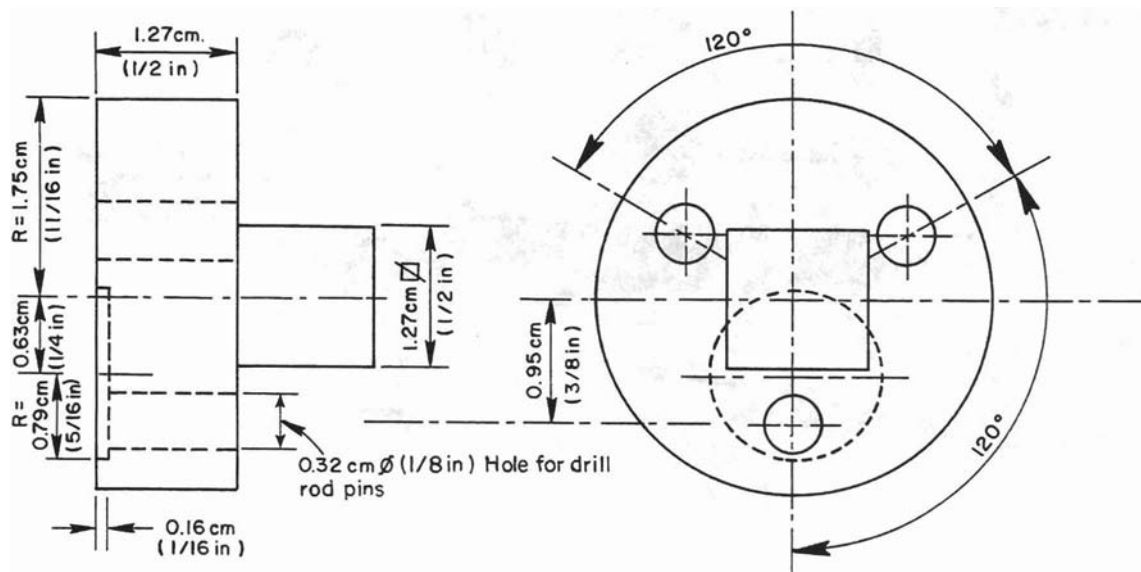
Figure B-10. Cylinder-Torque Adapter
