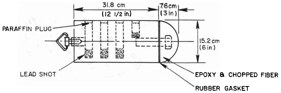
Figure B-2. Door Ram
