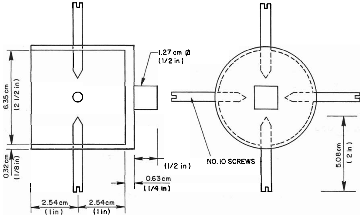
Figure B-9. Knob-Torque Adapter
