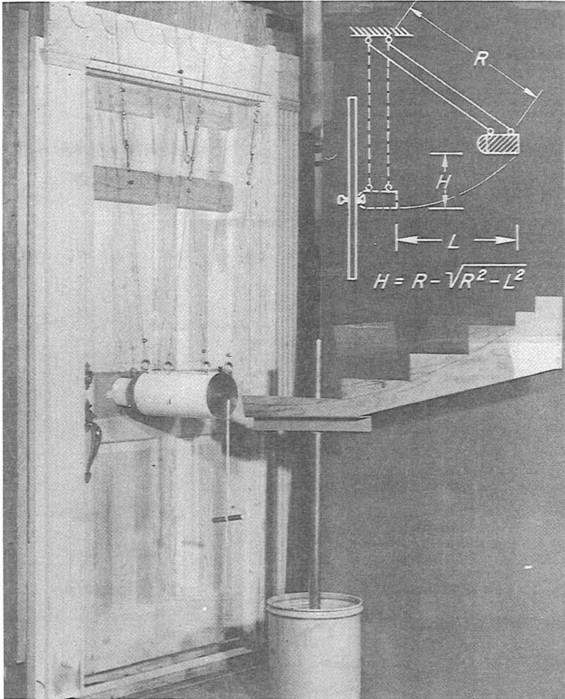
Figure B-1. Door Ram Pendulum System.
