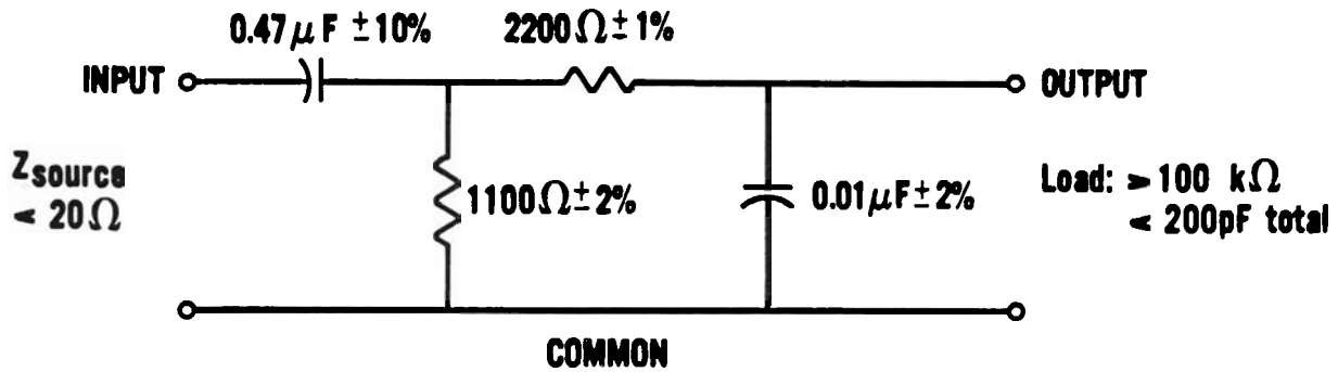
FIGURE 2. Noise filter circuit diagram.
