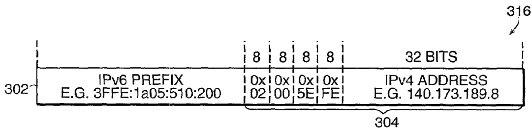
FIG. 15D IPv6-IPv4 COMPATIBILITY ADDRESS
