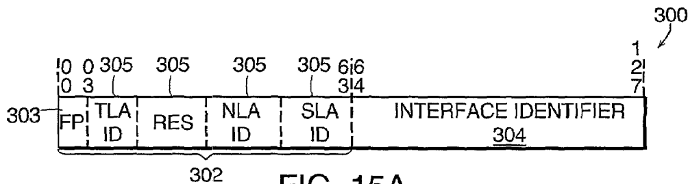
FIG. 15A IPv6-IPv4 COMPATIBILITY ADDRESS FORMAT
