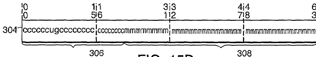
FIG. 15B INTERFACE IDENTIFIER FORMAT
