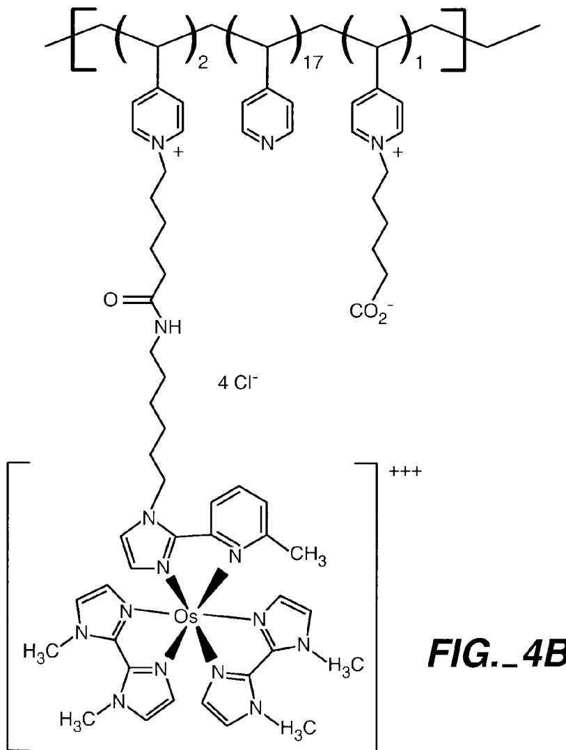
Structure of Redox Polymer 316
