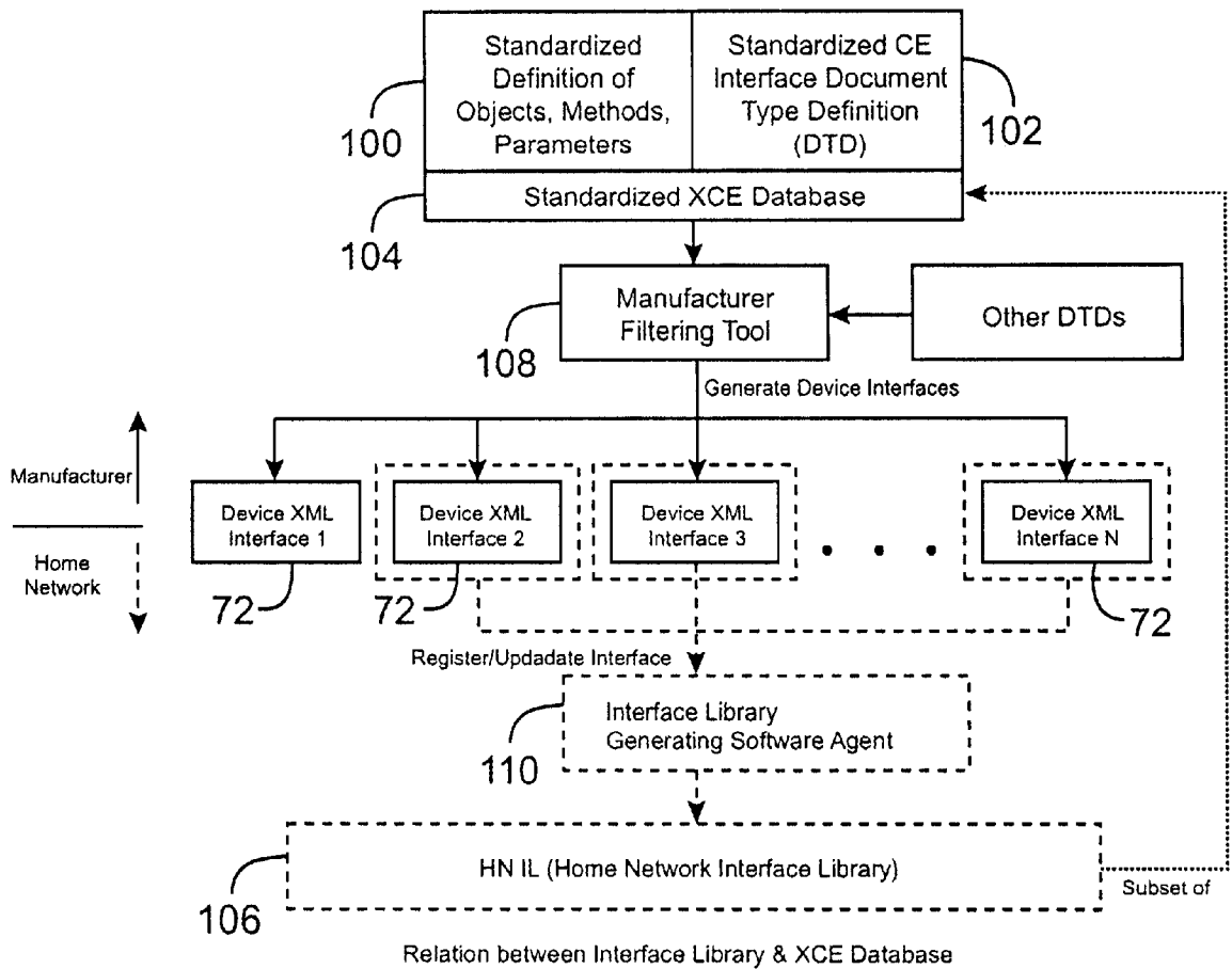
Relation between Interface Library & XCE Database
