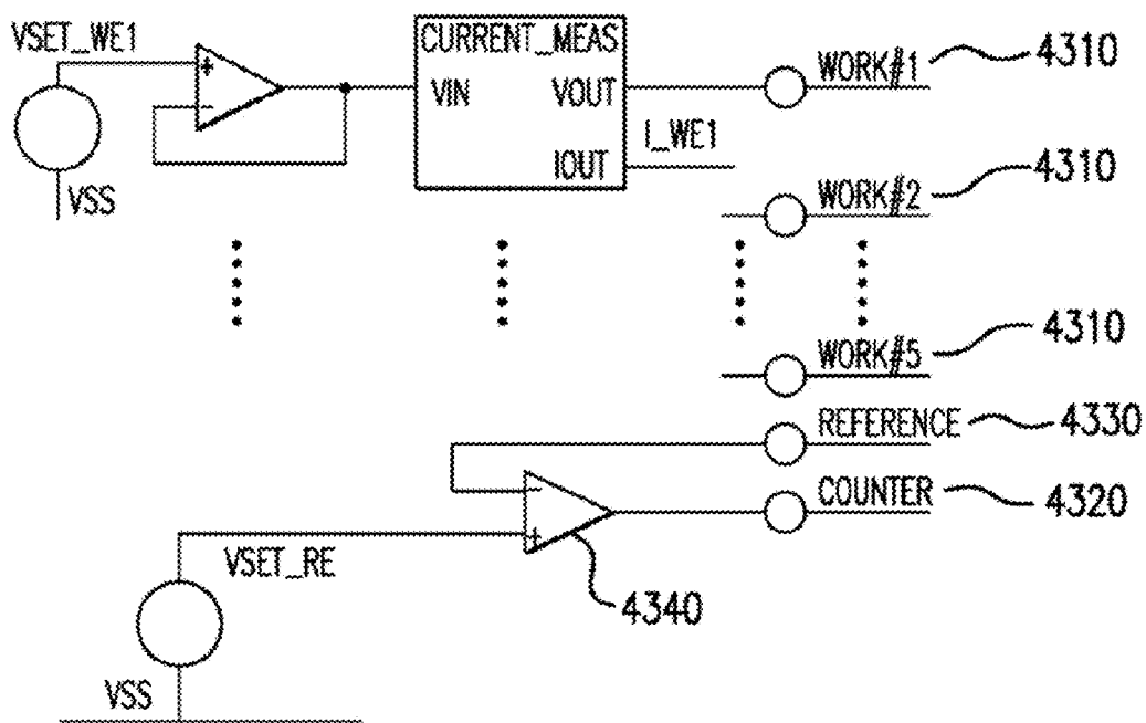
POTENTIOSTAT CONFIGURATION
