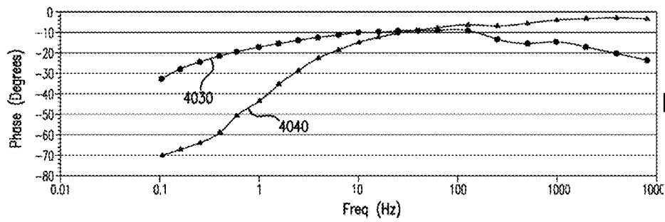
BODE PLOT- Before and After Cresol Added
