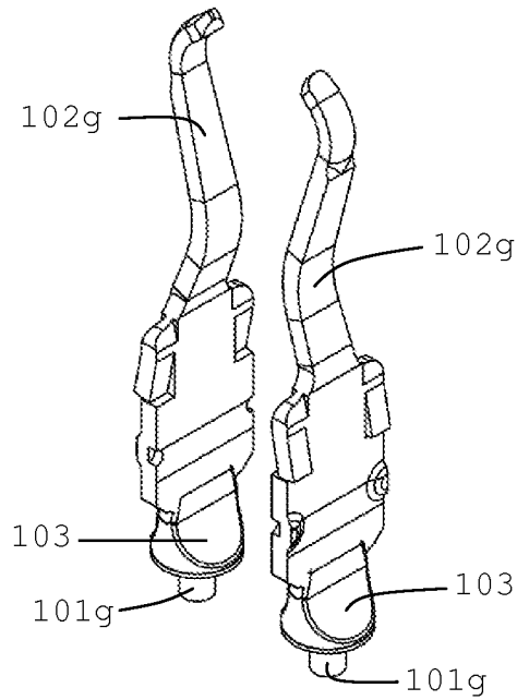
Fig. 20 PRIOR ART
