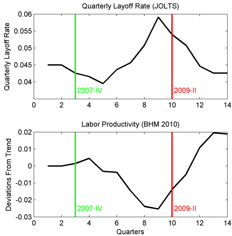
Figure 19: Forcing Variables
