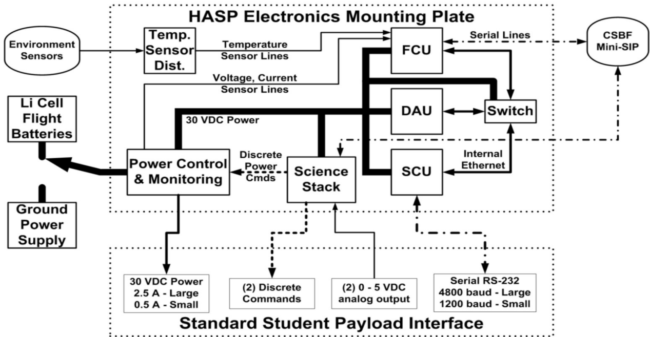
HASP flight electronics system and student payload interface
