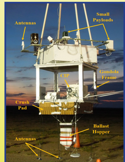
The HASP payload as configured for a typical flight (CIP: Consolidated Instrument Package)
