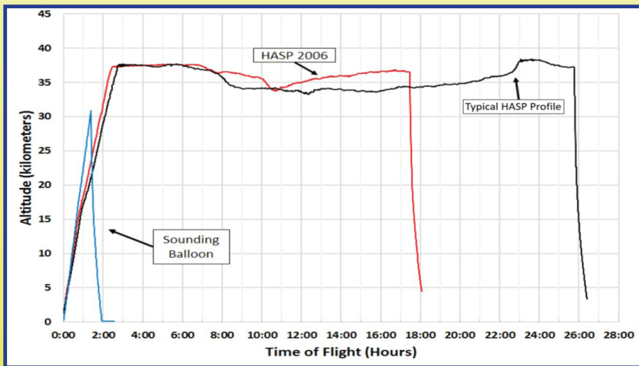
A typical altitude vs. time flight profile for HASP compared to that of a sounding balloon flight
