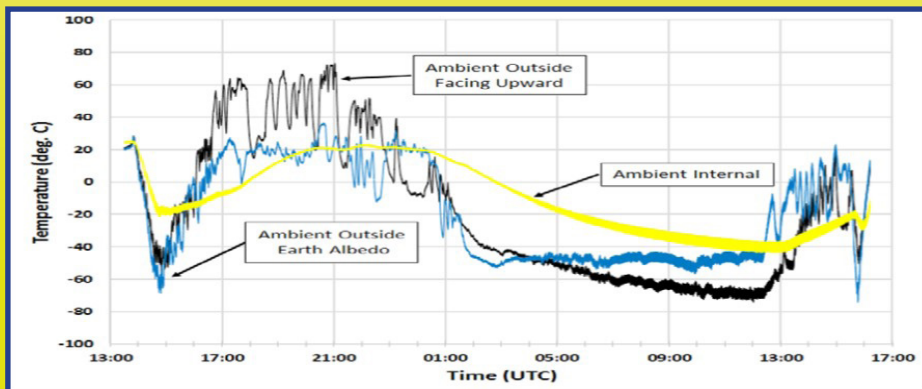
Characteristic temperatures outside HASP during flight
