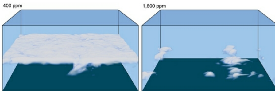
Fig. 2: results of modelling of marine stratocumulus behaviour in a high- \text{CO}_2 world. This one compares conditions at 400 ppm (present) and 1600 ppm (hopefully never, but relevant to the Palaeocene and Eocene when a super-Hothouse climate prevailed). Redrawn from Schneider et al. 2019 .
