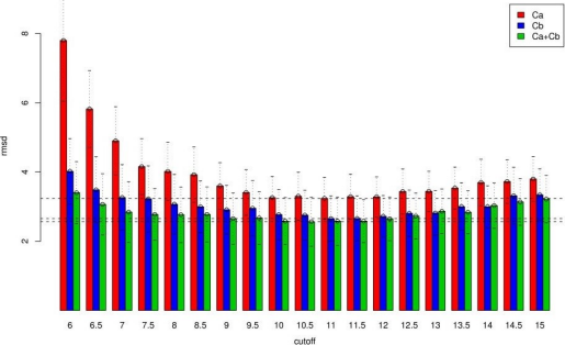
Average reconstruction for 60 PDB representatives
