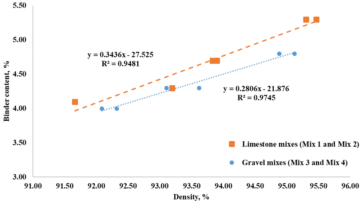
Figure 39. Relationships between Binder Contents and SGC Laboratory-Molded Densities at a Compaction Level of 75 Gyration.
