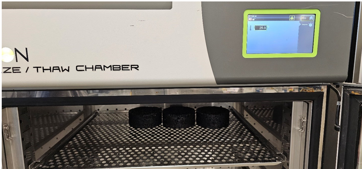
Figure 20. Conditioning of IDEAL-RT Specimens.
