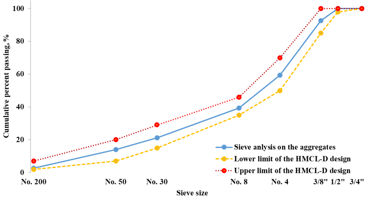
Figure 13. Aggregate Gradations of Gravel HMCL-D Mixes.
