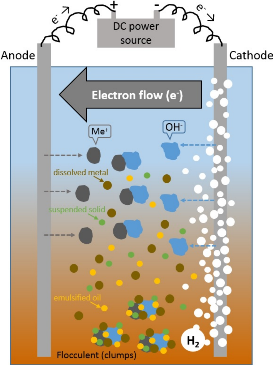
Figure 1. Electro-coagulation
