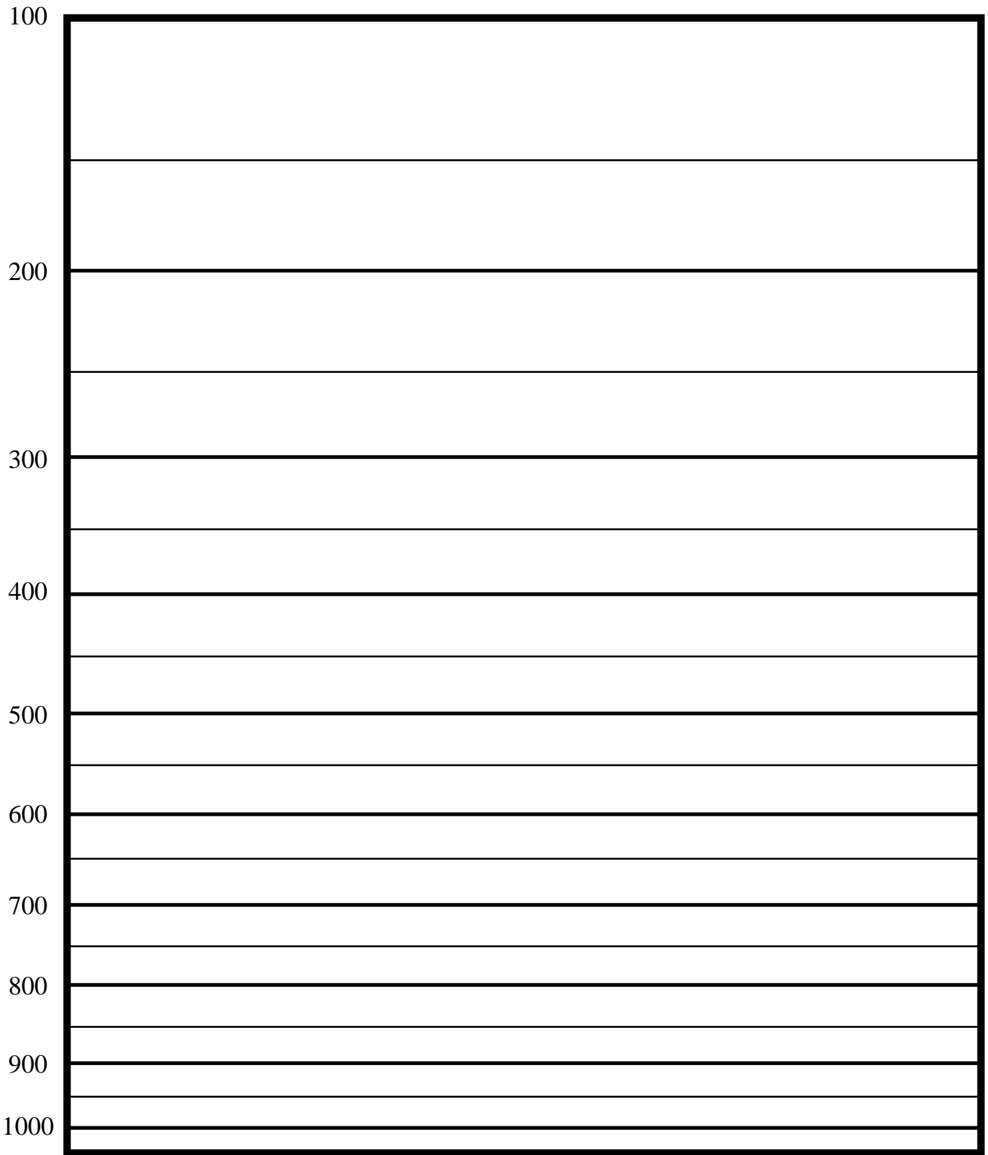
Isobars (Millibars)
