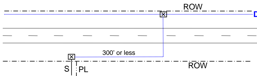
Figure 4: Long-side service connection plus distribution extension
