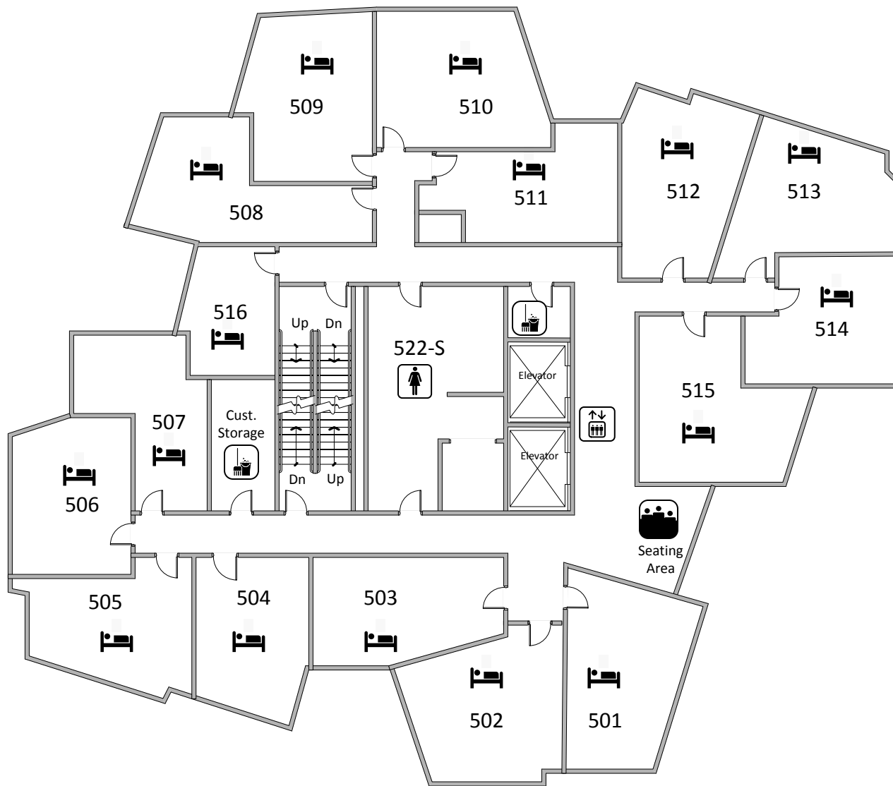
Level 5 Floor Plan No Scale
