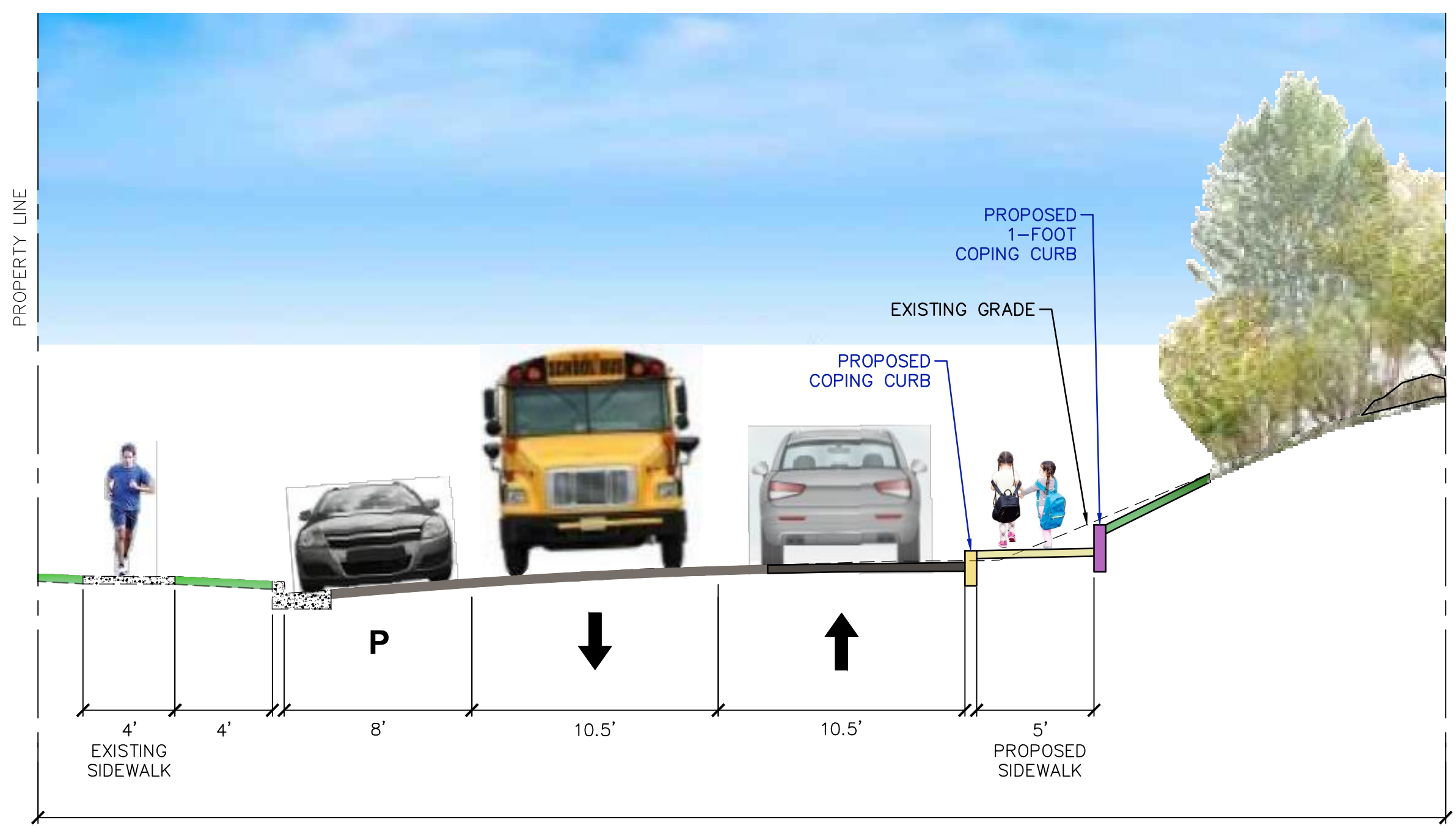
ILLUSTRATIVE CROSS SECTION A-A NOT TO SCALE
