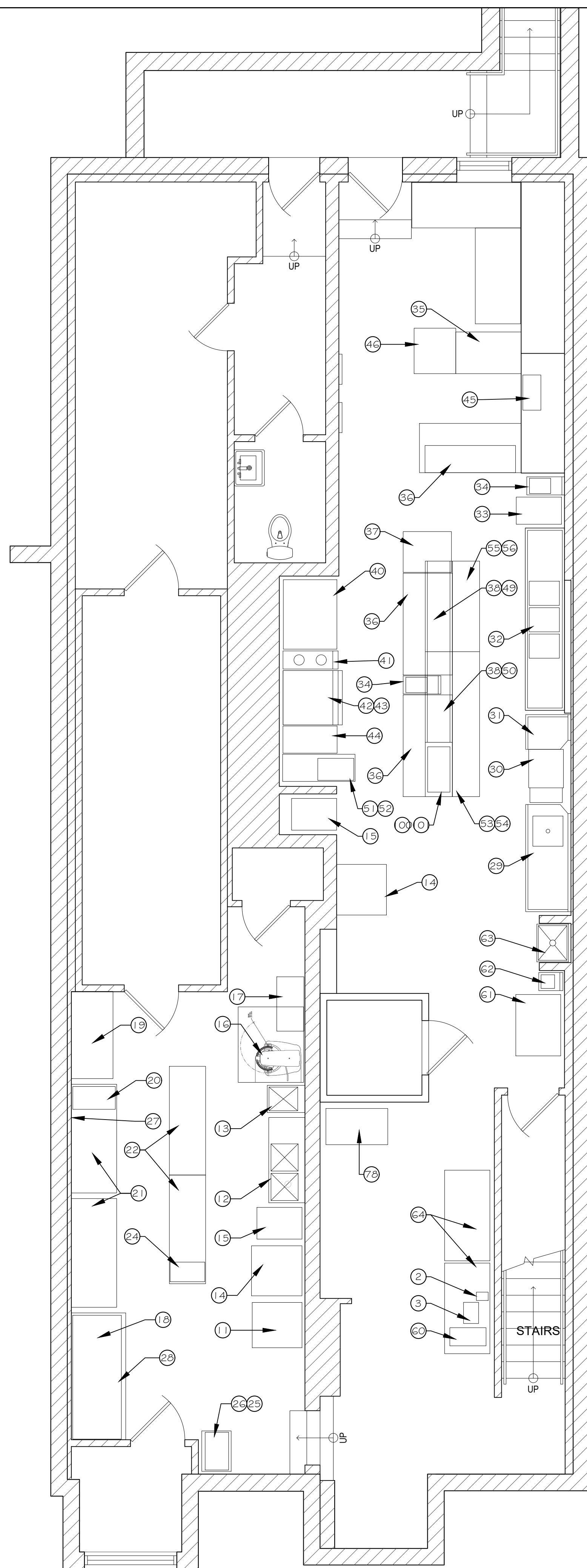
01 BASEMENT PROPOSED FLOOR PLAN SCALE: 1/4" = 1' - 0"
