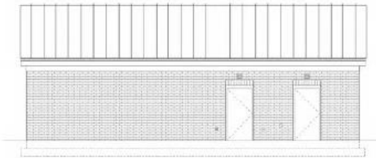
4 NORTH ELEVATION 1/8" = 1'-0"
