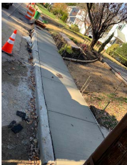
Figure 2: Concrete sidewalk
