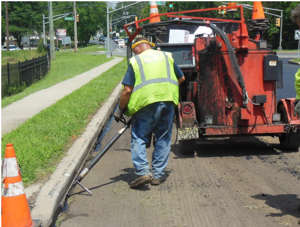
Figure 1 Installing tack along edge of curb
