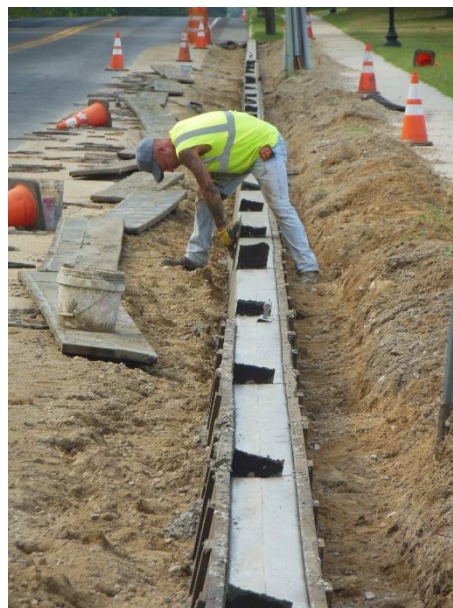
Figure 5 Contractor's removing forms from curb after concrete set up enough to finish face
