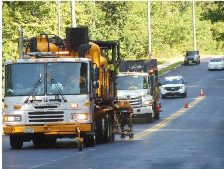
Figure 2 Sub-contractor Zone installing double yellow with GTPD assistants
