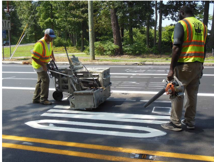
Figure 4 Installing thermo of an Only at Hickstown Road
