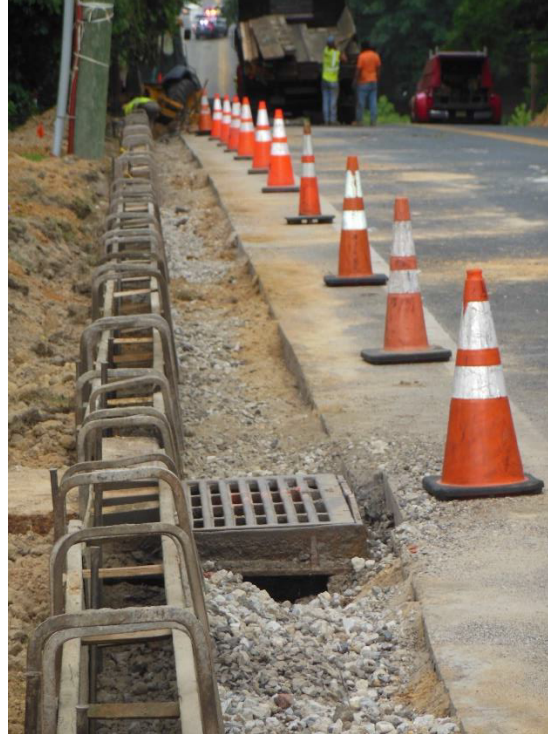
Figure 6 New curb forms ready to be poured
