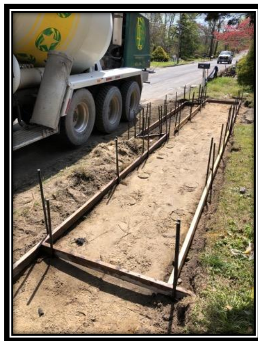
Figure: 3 – Installation of concrete driveway and sidewalk along the southbound lane of Watsontown-New Freedom Road (CR 691) between the White Horse Pike and Berlin-Clementon Road in the Borough of Clementon
