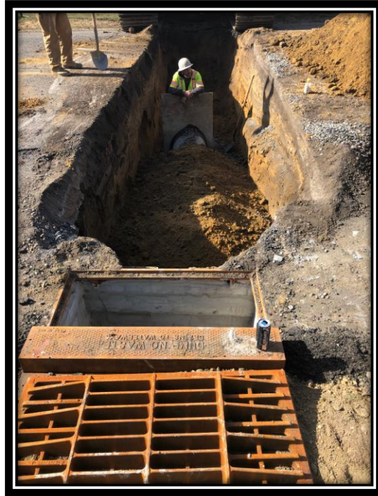
Figure: 2 – Installation of 18” RCP crossing on Watsontown-New Freedom Road (CR 691) between Carriage Stop Drive and Westbury Drive in the Boroughs of Berlin and Pine Hill
