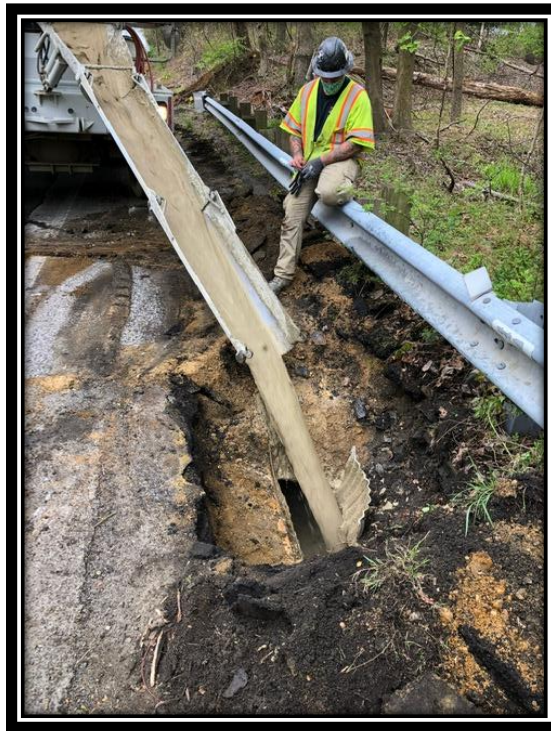
Figure: 3 – Installation of flowable fill into the existing 36" CMP storm sewer to be abandoned in place along the southbound lane of Watsontown-New Freedom Road (CR 691) between Berlin-Clementon Road and Carriage Stop Drive in the Borough of Pine Hill
