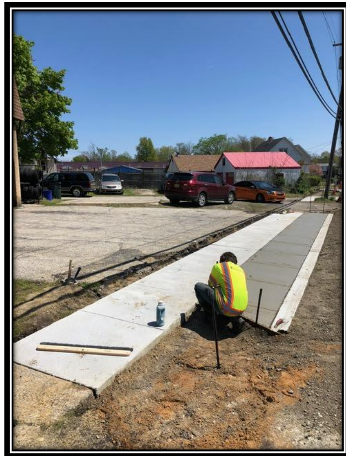
Figure: 1 – Installation of concrete curb, sidewalk and driveway apron along the northbound lane of Watsonstown-New Freedom Road (CR 691) in the Borough of Clementon
