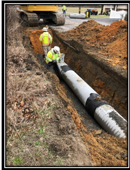
Figure: 2 – Installation of 18” RCP on Watsontown-New Freedom Road (CR 691) between Westbury Drive and Wyndam Road in the Borough of Berlin
