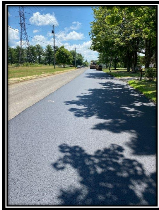
Figure: 3 – Installation of HMA 9.5M64 surface course along the southbound lane between Berlin-Clementon Road and Berlin-Cross Keys Road in the Borough of Pine Hill
