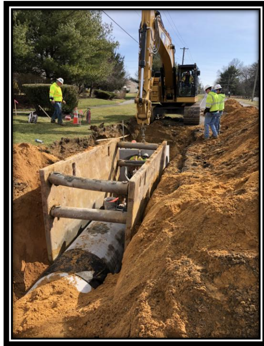
Figure: 2 – Installation of 36” RCP along the northbound lane of Watsontown-New Freedom Road (CR 691) in the Borough of Berlin
