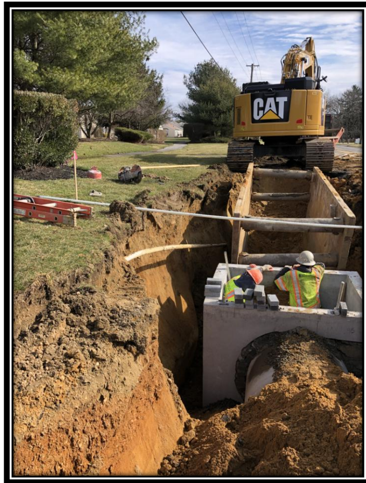
Figure: 1 – Installation of type B-2 inlet along the northbound lane of Watsonstown-New Freedom Road (CR 691) in the Borough of Berlin
