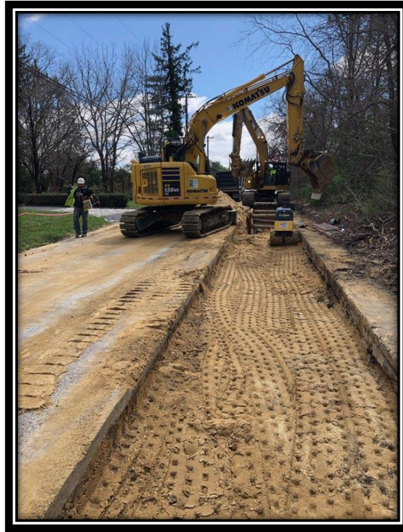
Figure: 2 – Backfill and compaction of the 36” RCP trench along the southbound lane of Watstown-New Freedom Road (CR 691) in the Borough of Pine Hill
