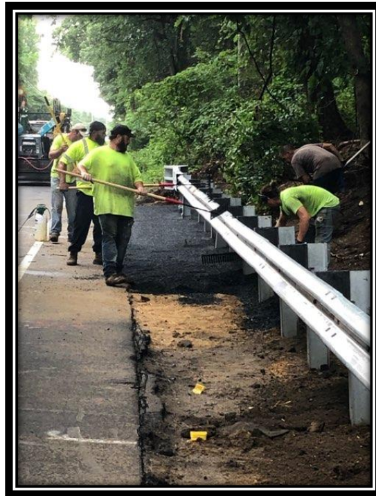
Figure: 3 – Installation of HMA non vegetative surface under the newly installed beam guide rail along the southbound lane between Berlin-Clementon Road and Carriage Stop Drive in the Borough of Pine Hill
