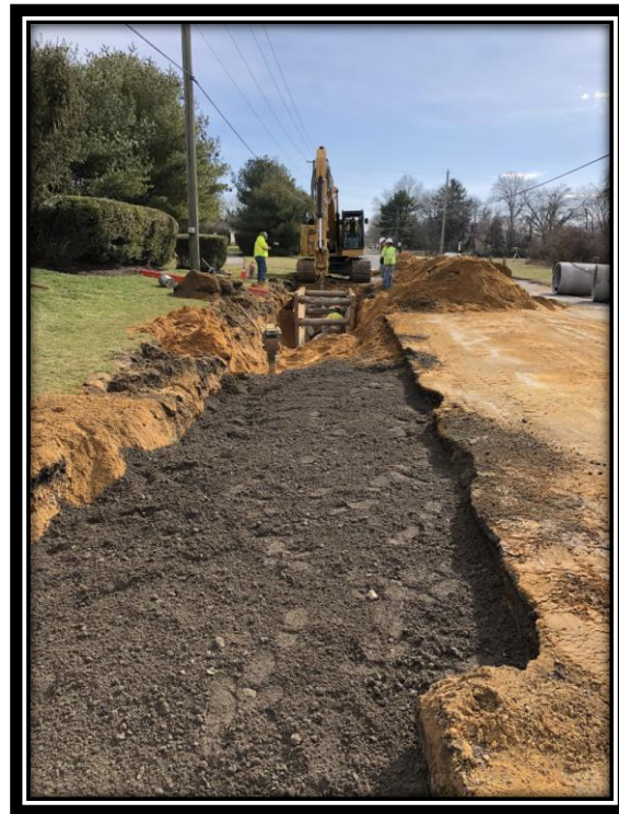
Figure: 3 – Restoration and compaction of the 36” RCP trench along the northbound lane of Watsontown-New Freedom Road (CR 691) in the Borough of Berlin
