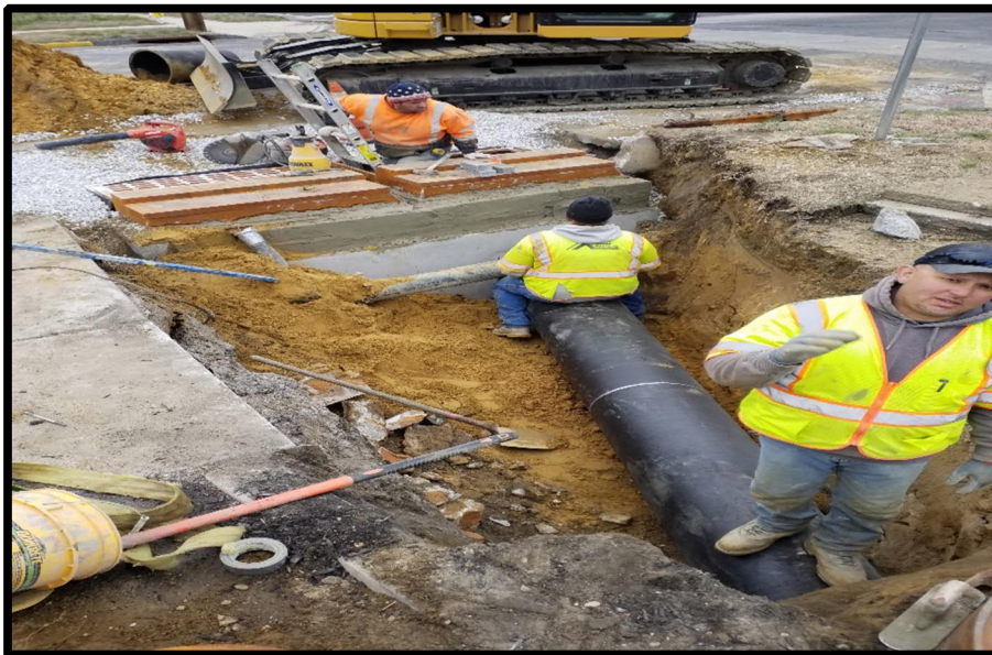
Photograph 3 – pipe Crew installing 18” ductile iron pipe.
