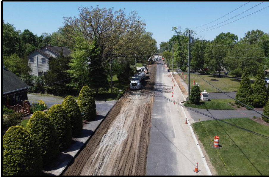
Photograph 6 – Full Depth reclamation Crew operation.
