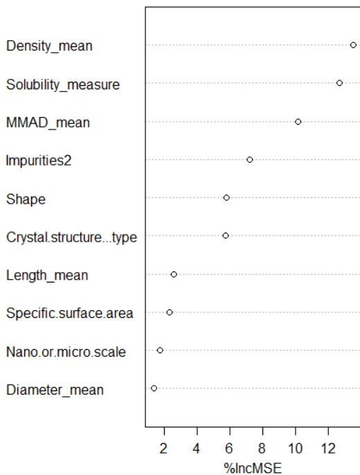
Figure 3-18: Estimated Variable Importance for Predicting the Inflammation Hierarchical Cluster for materials in the NTP histopathology data.
