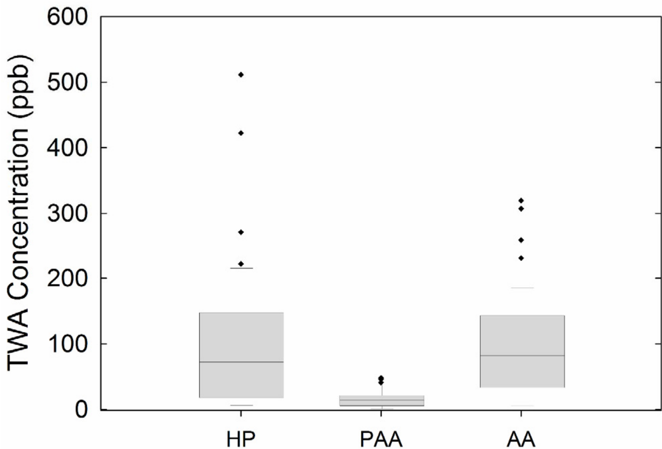
Figure 1. Box-plots of full-shift time-weighted average (TWA) exposure levels of hydrogen peroxide, peracetic acid, and acetic acid, NIOSH survey, July and September 2015. Note: ppb=parts per billion. The boxplots illustrate each quartile with the lowest quartile shown as the line and hatch mark below the box, the second and third quartiles indicated by the shaded box, and the highest quartile indicated by the line and hatch mark above the boxes. The line within each box indicates the median air sample concentration. Outlier air samples are denoted by dots. The OSHA PEL and NIOSH REL is 1000 ppb (1 ppm) for hydrogen peroxide and 10,000 ppb (10 ppm) for acetic acid.
