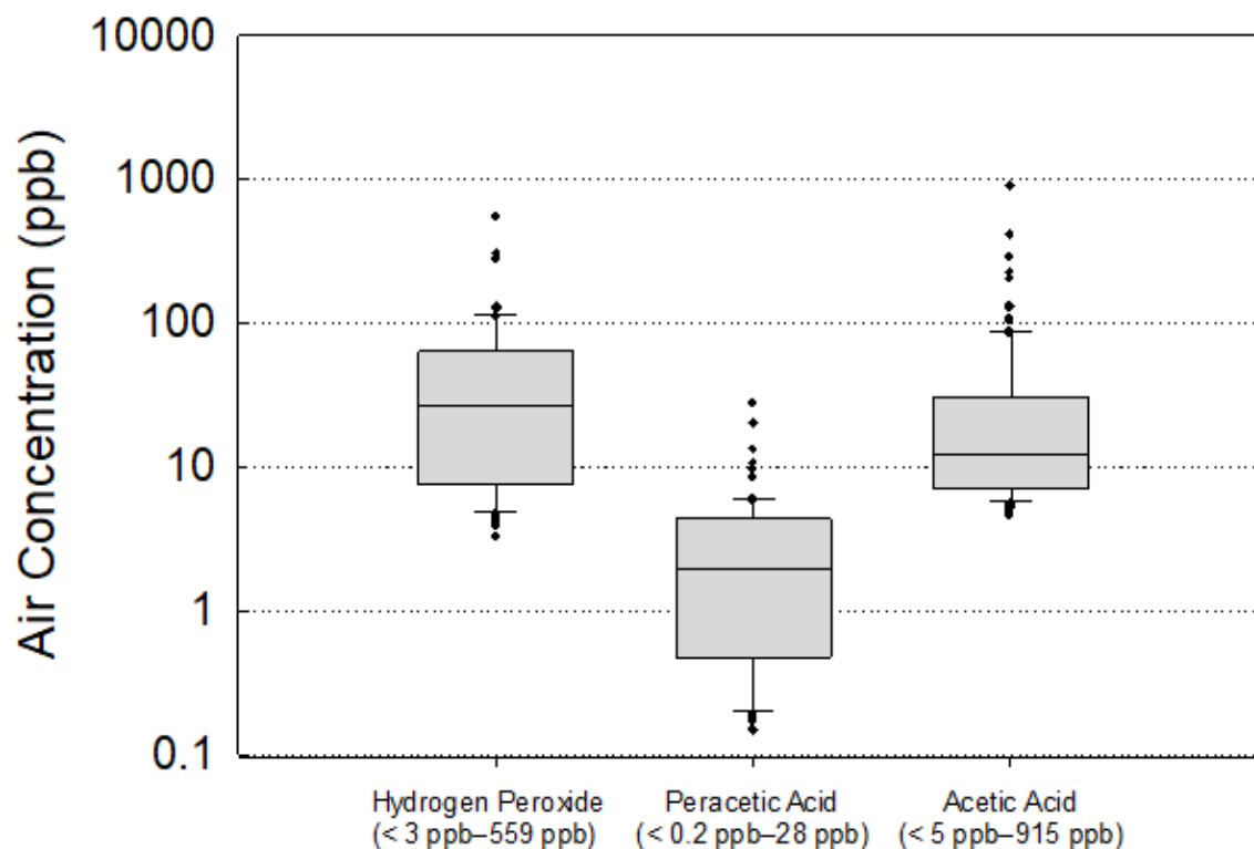
Figure 1. Box-plots of full-shift time-weighted average exposure levels of hydrogen peroxide (HP), peracetic acid (PAA), and acetic acid (AA), NIOSH survey, July and August 2018. Note: ppb=parts per billion. The box-plots illustrate each quartile with the lowest quartile shown as the line and hatch mark below the box, the second and third quartiles indicated by the shaded box, and the highest quartile indicated by the line and hatch mark above the boxes. The line within each box indicates the median air sample concentration. Outlier air samples are denoted by dots. The OSHA PEL and NIOSH REL is 1000 ppb (1 ppm) for hydrogen peroxide and 10,000 ppb (10 ppm) for acetic acid.
