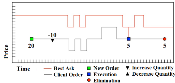
Figure 3.9: Example of Participant Order Trace Graph
