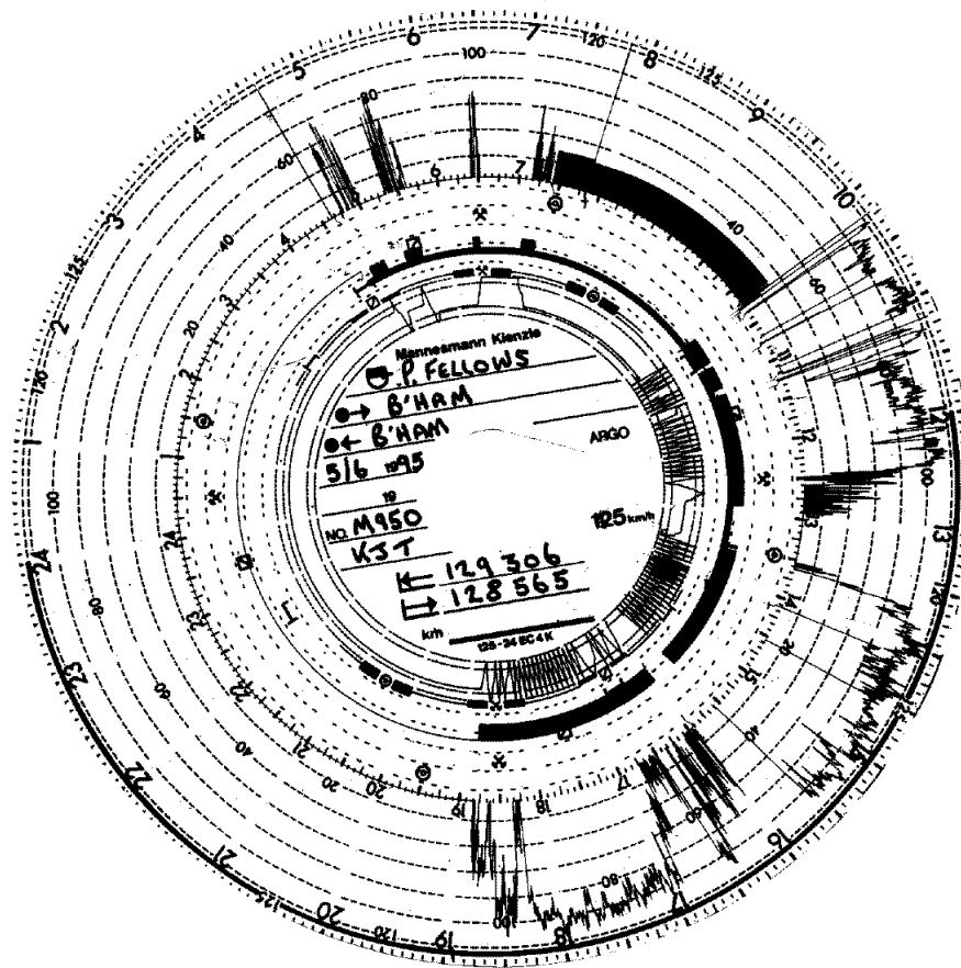
Figure 10.3: – a tachograph chart
