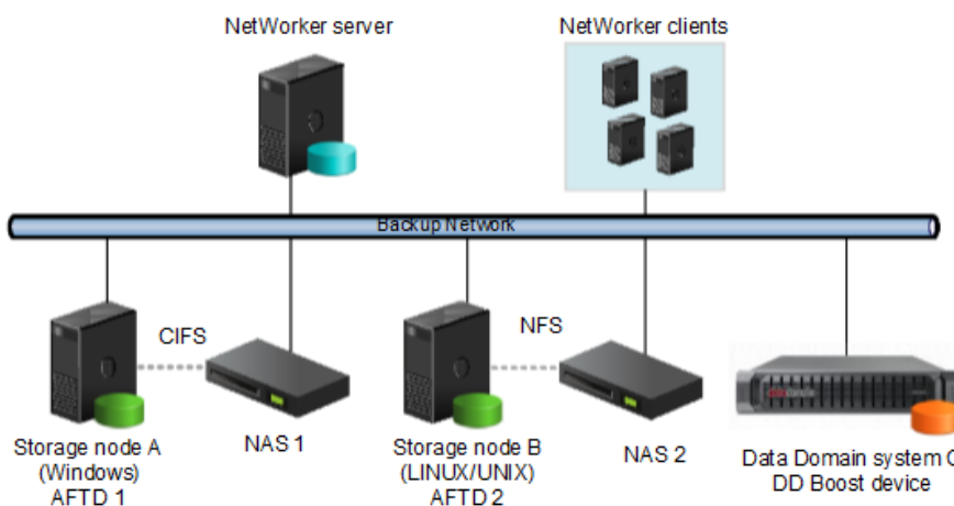
Figure 13 Example NetWorker disk backup configuration in a mixed backup environment.
