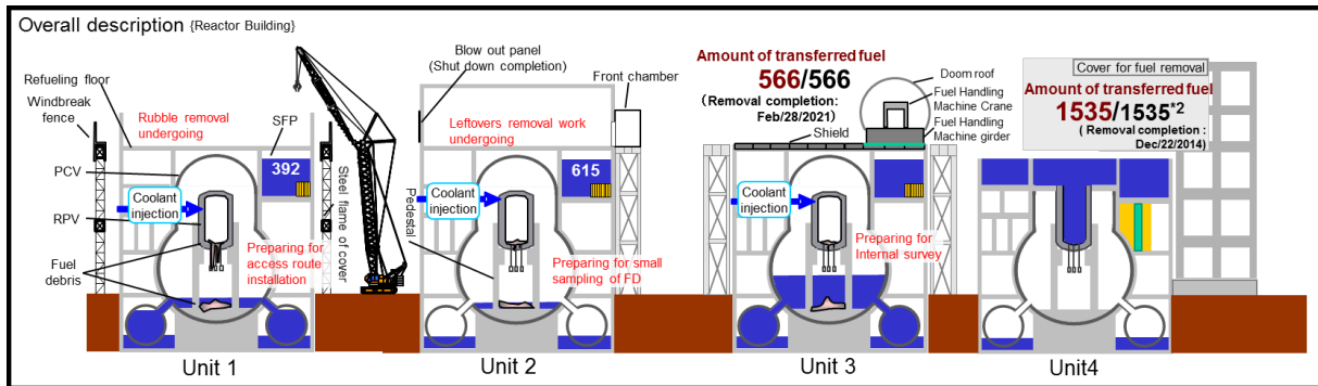
Figure 6. Status of spent fuel and fuel debris in Units 1-4 in July 2021 (courtesy by TEPCO).
