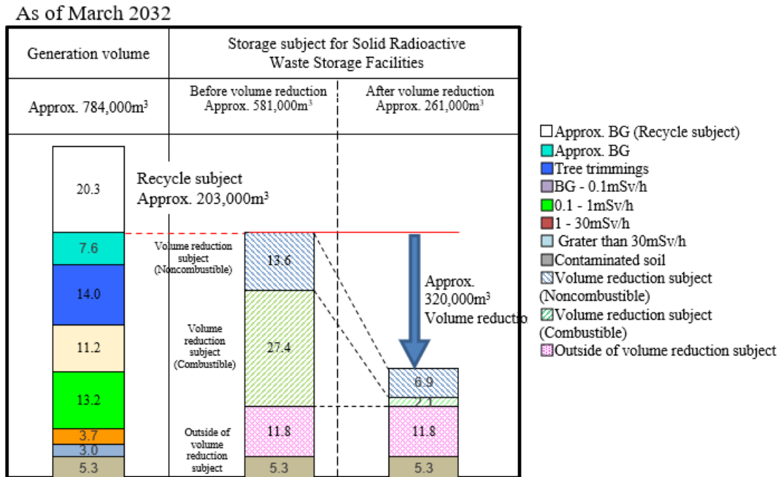
Figure 7. Forecast of volume of waste generated at Fukushima NPS through 2032 (courtesy of TEPCO).
