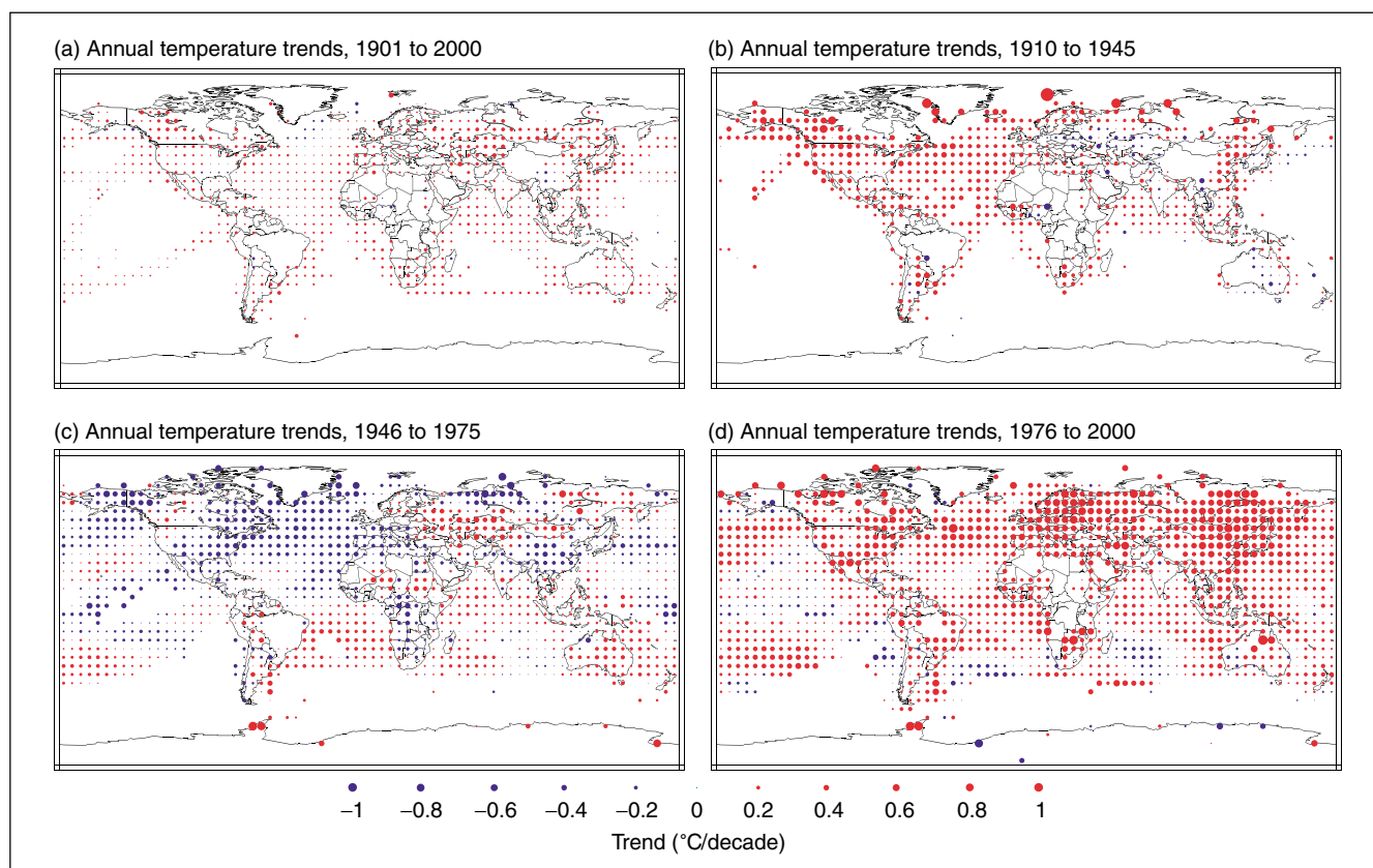
Figure 3: Annual temperature trends for the periods 1901 to 2000, 1910 to 1945, 1946 to 1975 and 1976 to 2000 respectively. Trends are represented by the area of the circle with red representing increases, blue representing decreases, and green little or no change. Trends were calculated from annually averaged gridded anomalies with the requirement that the calculation of annual anomalies include a minimum of 10 months of data. For the period 1901 to 2000, trends were calculated only for those grid boxes containing annual anomalies in at least 66 of the 100 years. The minimum number of years required for the shorter time periods (1910 to 1945, 1946 to 1975, and 1976 to 2000) was 24, 20, and 16 years respectively. [Based on Figure 2.9]
