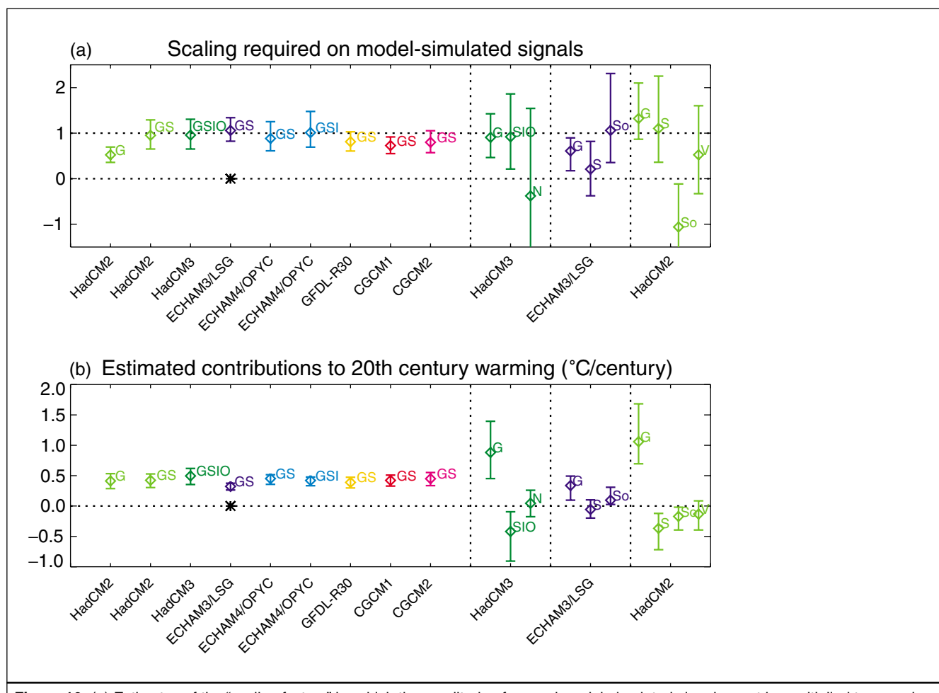
Figure 16: (a) Estimates of the “scaling factors” by which the amplitude of several model-simulated signals must be multiplied to reproduce the corresponding changes in the observed record. The vertical bars indicate the 5 to 95% uncertainty range due to internal variability. A range encompassing unity implies that this combination of forcing amplitude and model-simulated response is consistent with the corresponding observed change, while a range encompassing zero implies that this model-simulated signal is not detectable. Signals are defined as the ensemble mean response to external forcing expressed in large-scale (>5,000 km) near-surface temperatures over the 1946 to 1996 period relative to the 1896 to 1996 mean. The first entry (G) shows the scaling factor and 5 to 95% confidence interval obtained with the assumption that the observations consist only of a response to greenhouse gases plus internal variability. The range is significantly less than one (consistent with results from other models), meaning that models forced with greenhouse gases alone significantly over predict the observed warming signal. The next eight entries show scaling factors for model-simulated responses to greenhouse and sulphate forcing (GS), with two cases including indirect sulphate and tropospheric ozone forcing, one of these also including stratospheric ozone depletion (GSI and GSIO, respectively). All but one (CGCM1) of these ranges is consistent with unity. Hence there is little evidence that models are systematically over- or under-predicting the amplitude of the observed response under the assumption that model-simulated GS signals and internal variability are an adequate representation (i.e., that natural forcing has had little net impact on this diagnostic). Observed residual variability is consistent with this assumption in all but one case (ECHAM3, indicated by the asterisk). One is obliged to make this assumption to include models for which only a simulation of the anthropogenic response is available, but uncertainty estimates in these single signal cases are incomplete since they do not account for uncertainty in the naturally forced response. These ranges indicate, however, the high level of confidence with which internal variability, as simulated by these various models, can be rejected as an explanation of recent near-surface temperature change. A more complete uncertainty analysis is provided by the next three entries, which show corresponding scaling factors on individual greenhouse (G), sulphate (S), solar-plus-volcanic (N), solar-only (So) and volcanic-only (V) signals for those cases in which the relevant simulations have been performed. In these cases, multiple factors are estimated simultaneously to account for uncertainty in the amplitude of the naturally forced response. The uncertainties increase but the greenhouse signal remains consistently detectable. In one case (ECHAM3) the model appears to be overestimating the greenhouse response (scaling range in the G signal inconsistent with unity), but this result is sensitive to which component of the control is used to define the detection space. It is also not known how it would respond to the inclusion of a volcanic signal. In cases where both solar and volcanic forcing is included (HadCM2 and HadCM3), G and S signals remain detectable and consistent with unity independent of whether natural signals are estimated jointly or separately (allowing for different errors in S and V responses). (b) Estimated contributions to global mean warming over the 20th century, based on the results shown in (a), with 5 to 95% confidence intervals. Although the estimates vary depending on which model’s signal and what forcing is assumed, and are less certain if more than one signal is estimated, all show a significant contribution from anthropogenic climate change to 20th century warming. [Based on Figure 12.12]
