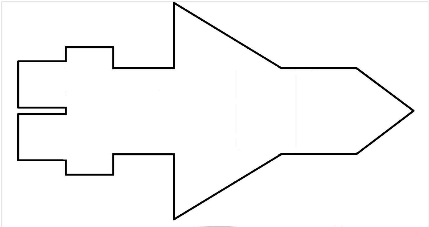
Tangram Rocket
