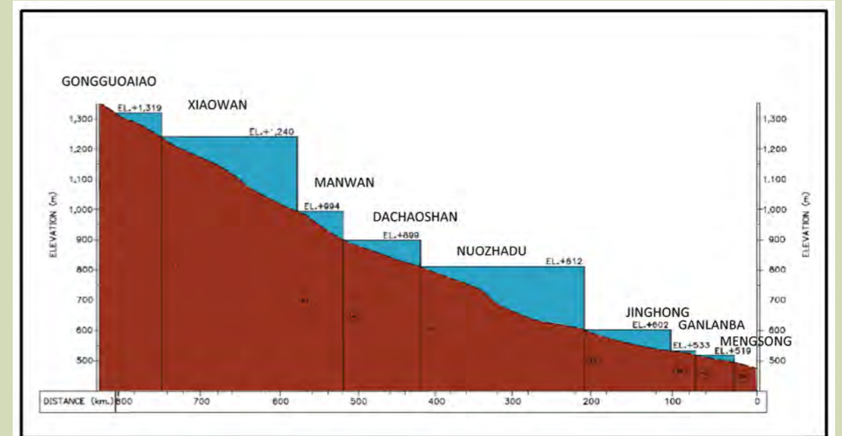
Figure 7.1 Profile of the hydropower cascade on the Lancang in China
