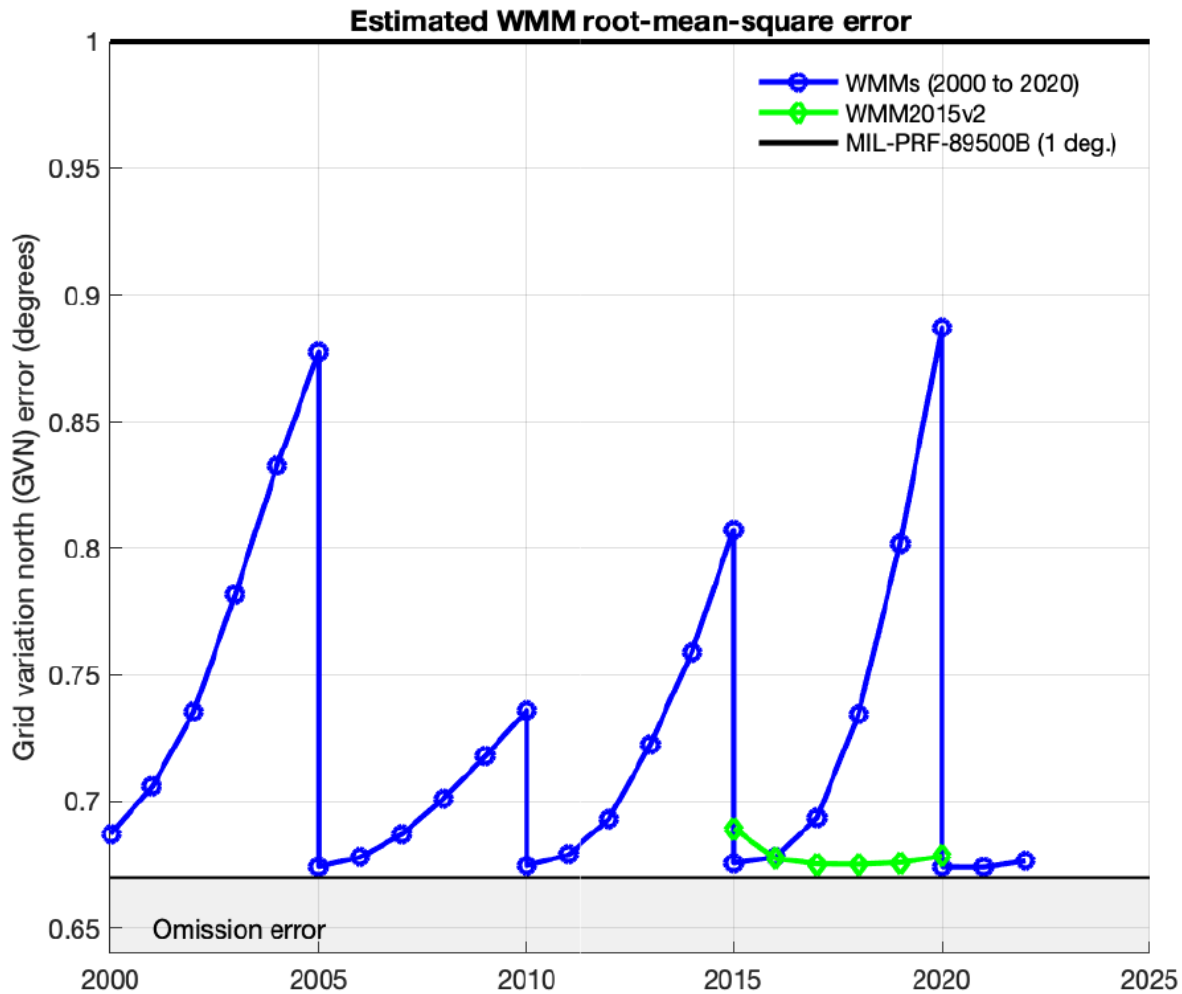
Figure 1: WMM global RMSE for the grid variation north (GVN) component from 2000 to 2022. Errors for six successive WMMs are shown: WMM2000, WMM2005, WMM2010, WMM2015, WMM2015v2 and WMM2020. WMM2015v2 was an out-of-cycle WMM released in late 2018 in case the WMM2015 were to breach the specification before the end of the cycle. (The specification was revised in 2019 with the introduction of so-called blackout zones, see below; blackout zones are no longer considered in WMM error calculations.)
