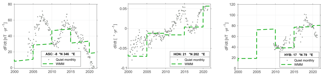
Figure 3: Observed rate of change of (a) field intensity ( F ) in nT/year at Ascension Island, South Atlantic (ASC), (b) rate of change of inclination angle ( I ) at Honolulu, Hawai'i, United States (HON) and (c) rate of change of field intensity ( F ) at Hyderabad, India (HYB). Quiet-dark monthly mean data are shown as grey circles, WMM predictions (WMM2000, WMM2005, WMM2010, WMM2015v2, WMM2020) are shown by the green dashed line.
