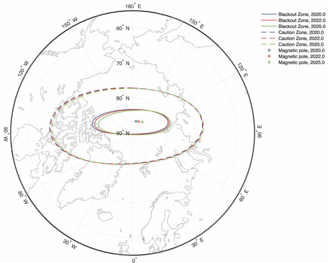
Figure 4: Successive locations of the magnetic dip pole, Blackout Zone and Caution Zone in the northern hemisphere throughout the WMM2020 five-year cycle.
