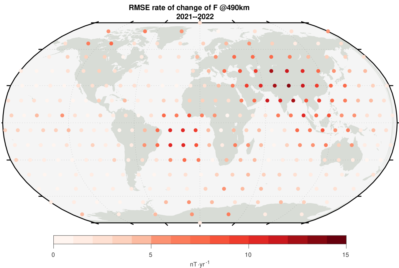
Figure 2: RMSE between prediction of WMM2020 SV of total intensity ( F ) and geomagnetic virtual observatory data in 2021.
