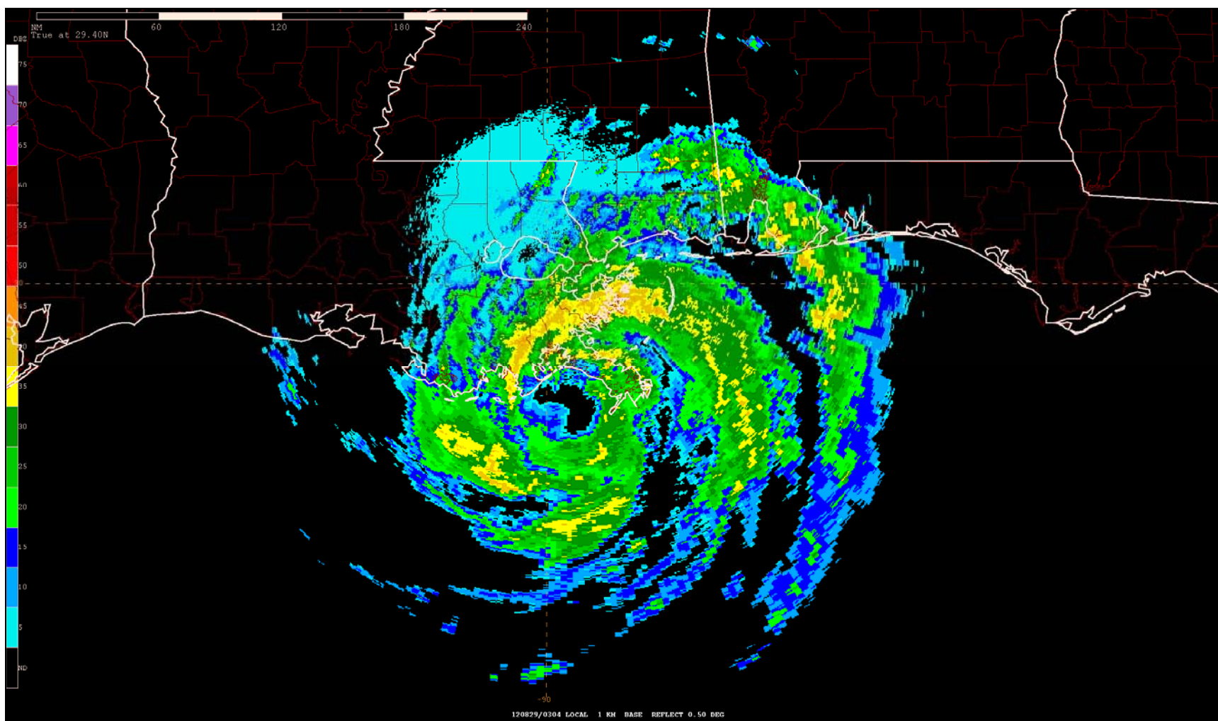
Figure 5. Radar image of Hurricane Isaac from the WSR-88D radar in Slidell, Louisiana, at 0304 UTC 29 August 2012 between its two landfalls along the coast of Louisiana. Isaac's minimum pressure of 965 mb is estimated to have occurred at this time.
